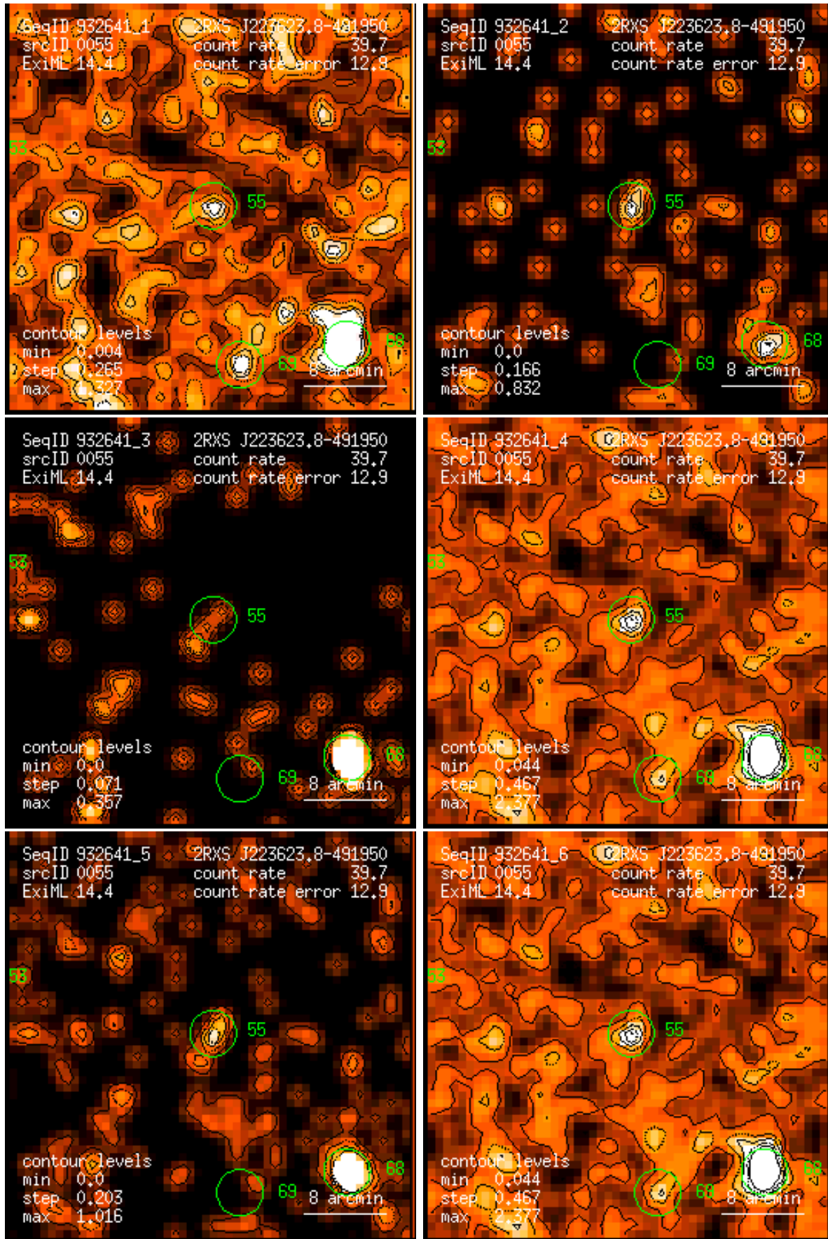
Figure 55: RASS 932641: detection 0055: band rate images, Gaussian filter: (1) PSPC channels 11 – 41, (2) 52 – 90, (3) 91 – 201, (4) 11 – 235, (5) 52 – 201, (6) 11 – 201. Broad band rates in counts/ks. Band rate contour levels in counts/ks/arcmin 2 .
