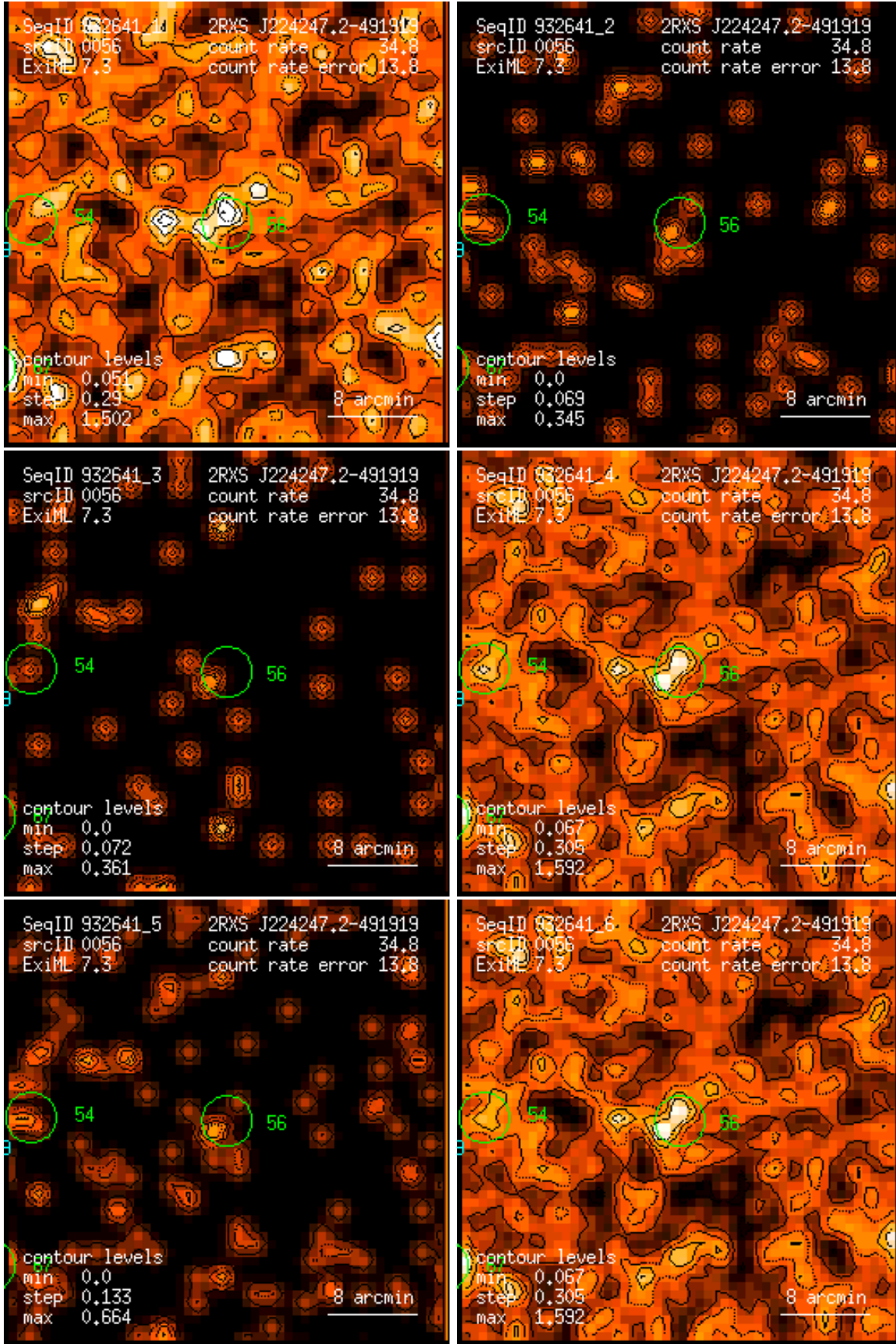
Figure 56: RASS 932641: detection 0056: band rate images, Gaussian filter: (1) PSPC channels 11 – 41, (2) 52 – 90, (3) 91 – 201, (4) 11 – 235, (5) 52 – 201, (6) 11 – 201. Broad band rates in counts/ks. Band rate contour levels in counts/ks/arcmin 2 .
