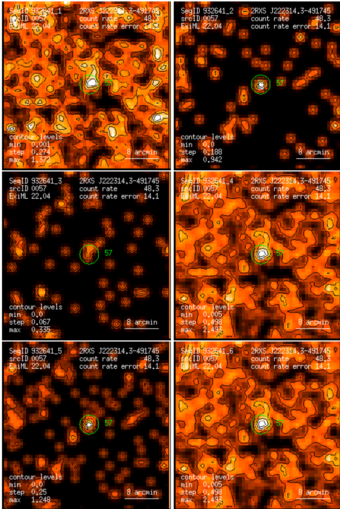
Figure 57: RASS 932641: detection 0057: band rate images, Gaussian filter: (1) PSPC channels 11 – 41, (2) 52 – 90, (3) 91 – 201, (4) 11 – 235, (5) 52 – 201, (6) 11 – 201. Broad band rates in counts/ks. Band rate contour levels in counts/ks/arcmin 2 .
