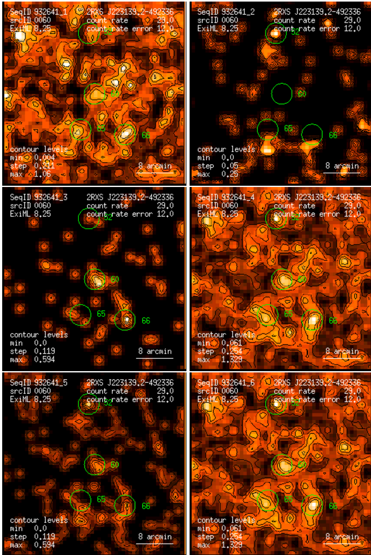
Figure 60: RASS 932641: detection 0060: band rate images, Gaussian filter: (1) PSPC channels 11 – 41, (2) 52 – 90, (3) 91 – 201, (4) 11 – 235, (5) 52 – 201, (6) 11 – 201. Broad band rates in counts/ks. Band rate contour levels in counts/ks/arcmin 2 .
