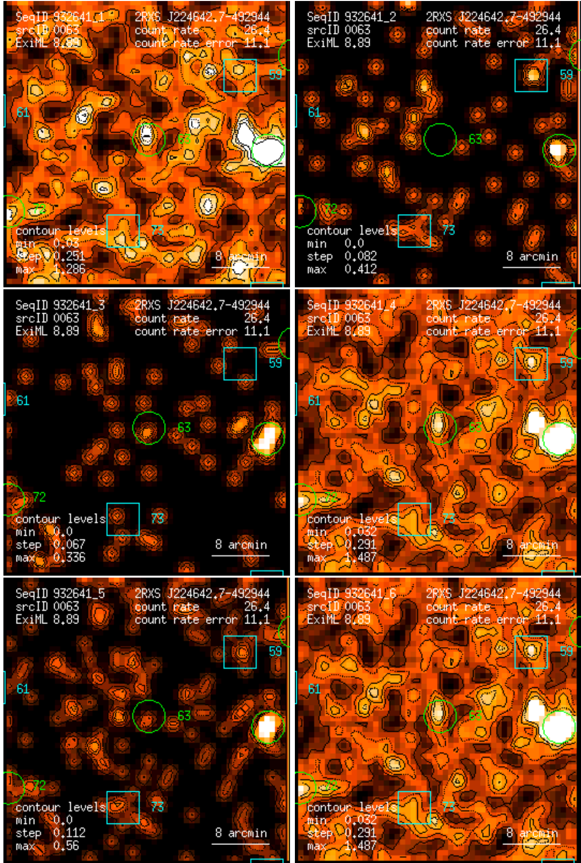
Figure 63: RASS 932641: detection 0063: band rate images, Gaussian filter: (1) PSPC channels 11 – 41, (2) 52 – 90, (3) 91 – 201, (4) 11 – 235, (5) 52 – 201, (6) 11 – 201. Broad band rates in counts/ks. Band rate contour levels in counts/ks/arcmin 2 .
