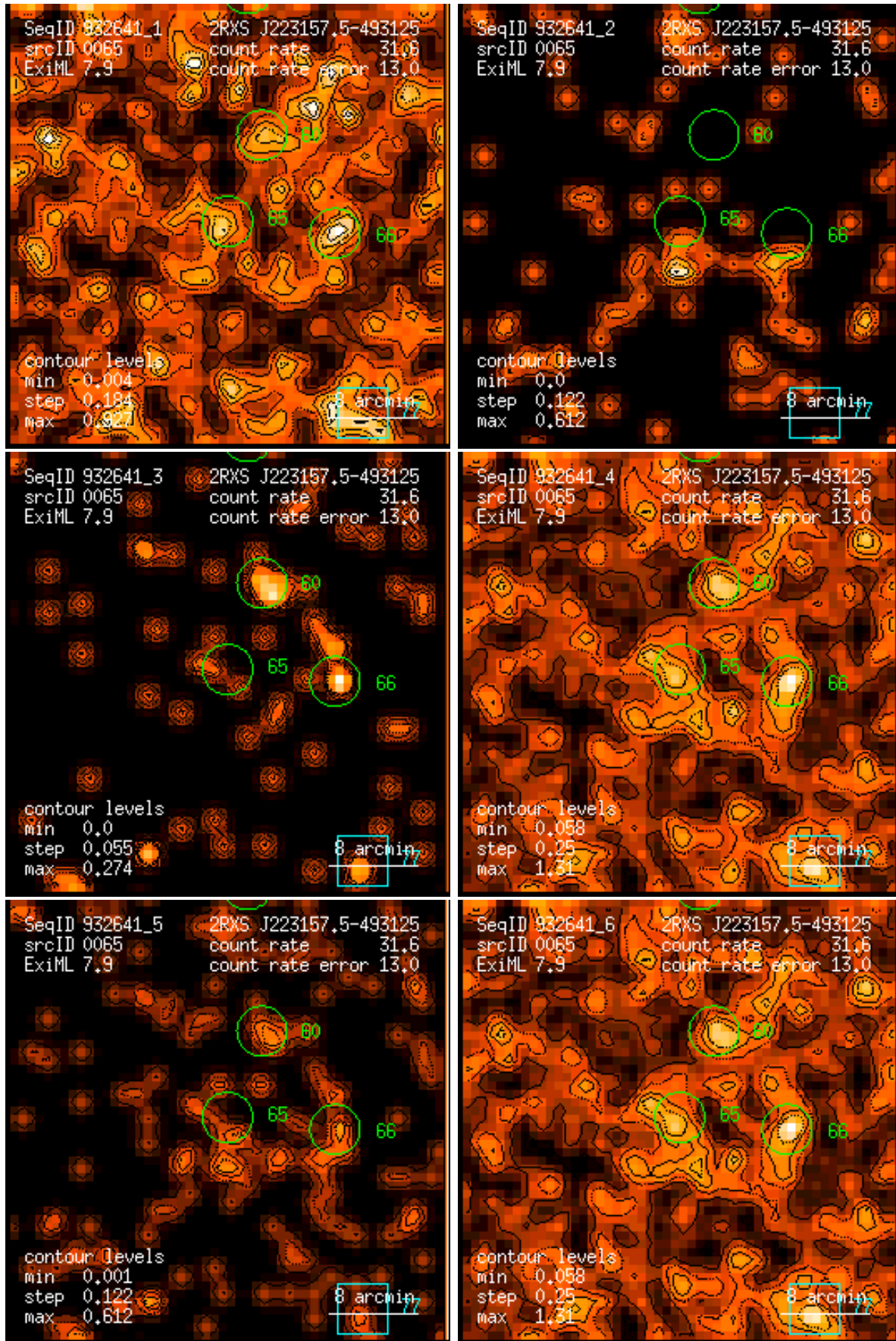
Figure 65: RASS 932641: detection 0065: band rate images, Gaussian filter: (1) PSPC channels 11 – 41, (2) 52 – 90, (3) 91 – 201, (4) 11 – 235, (5) 52 – 201, (6) 11 – 201. Broad band rates in counts/ks. Band rate contour levels in counts/ks/arcmin 2 .
