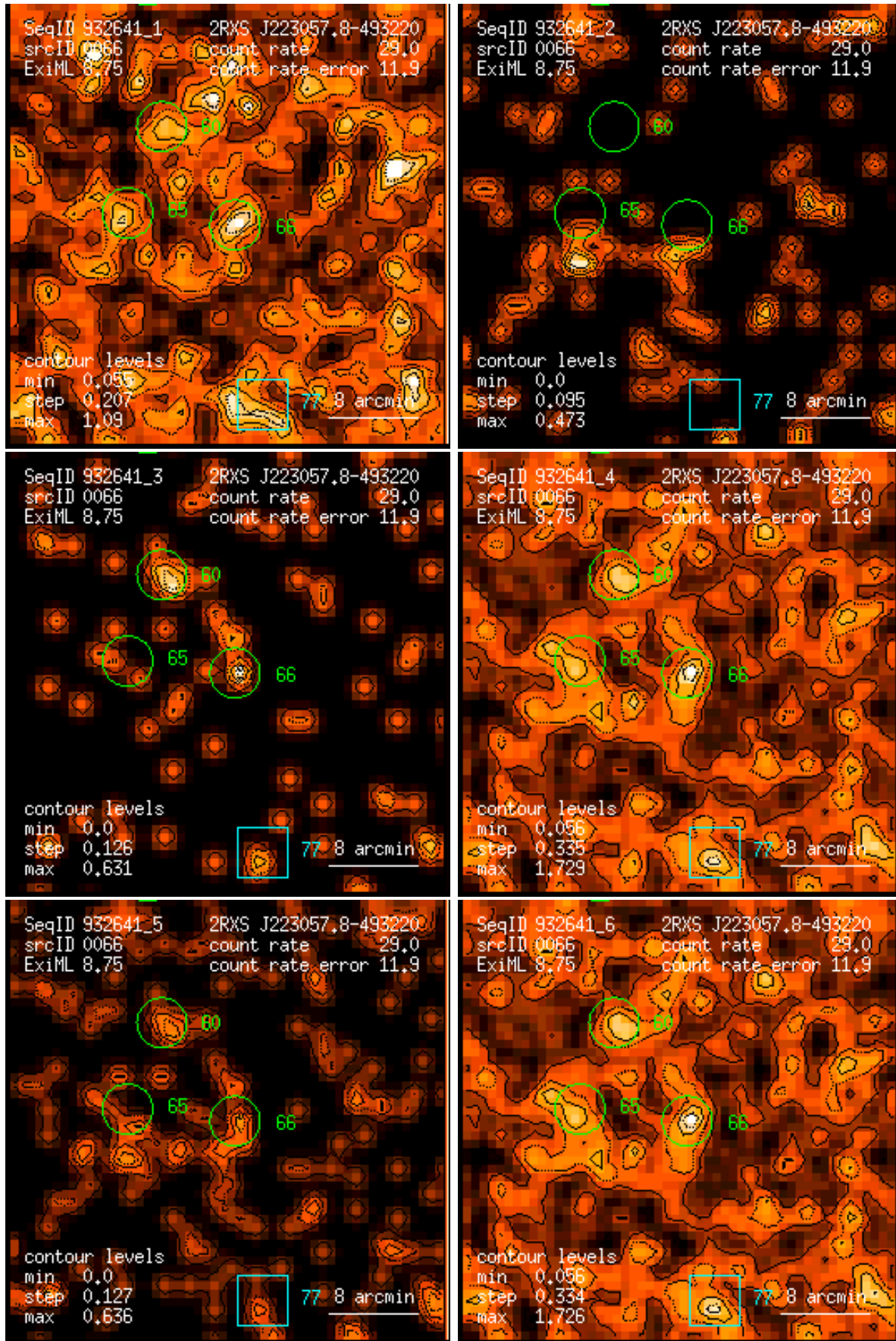
Figure 66: RASS 932641: detection 0066: band rate images, Gaussian filter: (1) PSPC channels 11 – 41, (2) 52 – 90, (3) 91 – 201, (4) 11 – 235, (5) 52 – 201, (6) 11 – 201. Broad band rates in counts/ks. Band rate contour levels in counts/ks/arcmin 2 .
