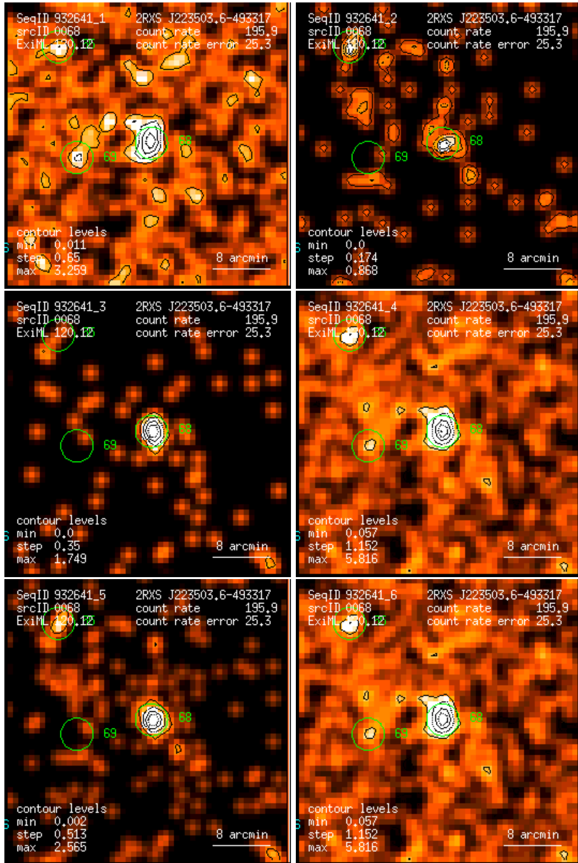
Figure 68: RASS 932641: detection 0068: band rate images, Gaussian filter: (1) PSPC channels 11 – 41, (2) 52 – 90, (3) 91 – 201, (4) 11 – 235, (5) 52 – 201, (6) 11 – 201. Broad band rates in counts/ks. Band rate contour levels in counts/ks/arcmin 2 .
