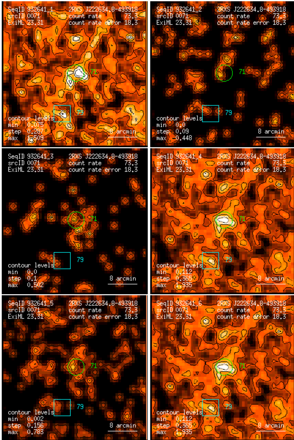
Figure 71: RASS 932641: detection 0071: band rate images, Gaussian filter: (1) PSPC channels 11 – 41, (2) 52 – 90, (3) 91 – 201, (4) 11 – 235, (5) 52 – 201, (6) 11 – 201. Broad band rates in counts/ks. Band rate contour levels in counts/ks/arcmin 2 .
