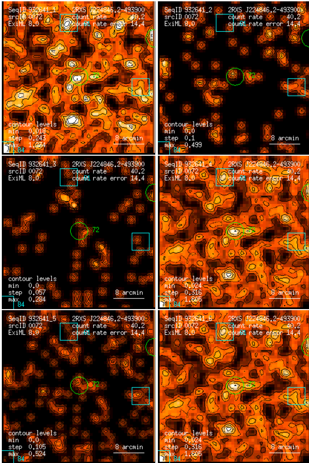
Figure 72: RASS 932641: detection 0072: band rate images, Gaussian filter: (1) PSPC channels 11 – 41, (2) 52 – 90, (3) 91 – 201, (4) 11 – 235, (5) 52 – 201, (6) 11 – 201. Broad band rates in counts/ks. Band rate contour levels in counts/ks/arcmin 2 .
