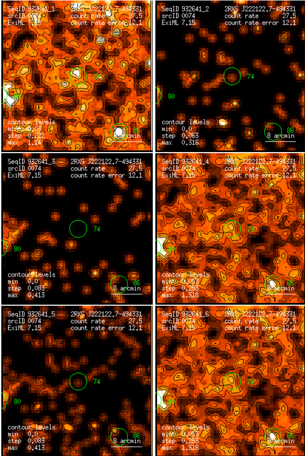
Figure 74: RASS 932641: detection 0074: band rate images, Gaussian filter: (1) PSPC channels 11 – 41, (2) 52 – 90, (3) 91 – 201, (4) 11 – 235, (5) 52 – 201, (6) 11 – 201. Broad band rates in counts/ks. Band rate contour levels in counts/ks/arcmin 2 .
