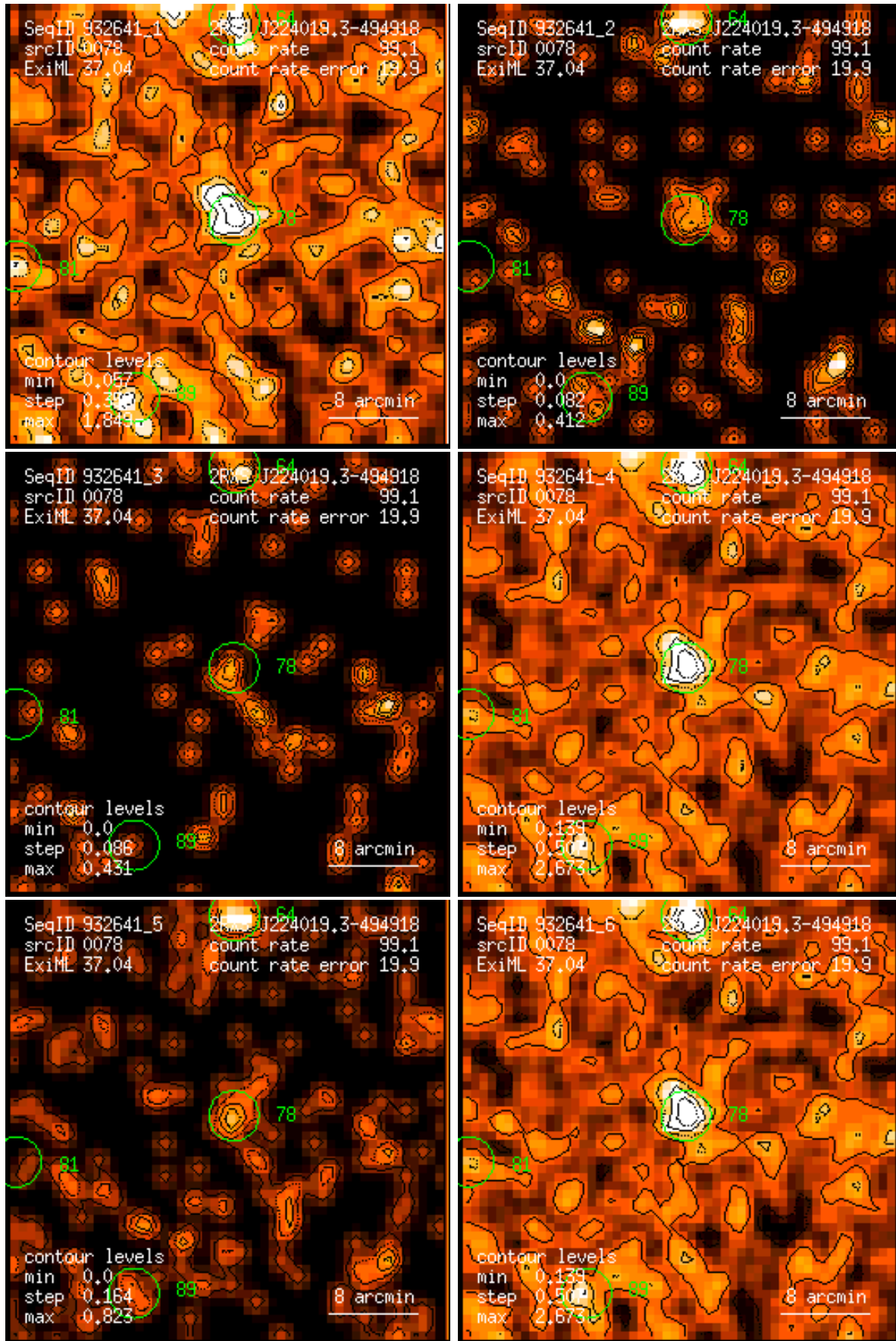
Figure 78: RASS 932641: detection 0078: band rate images, Gaussian filter: (1) PSPC channels 11 – 41, (2) 52 – 90, (3) 91 – 201, (4) 11 – 235, (5) 52 – 201, (6) 11 – 201. Broad band rates in counts/ks. Band rate contour levels in counts/ks/arcmin 2 .
