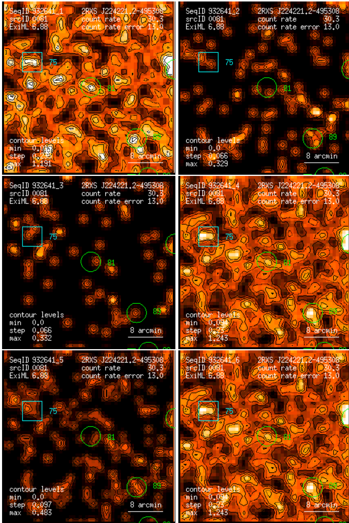
Figure 81: RASS 932641: detection 0081: band rate images, Gaussian filter: (1) PSPC channels 11 – 41, (2) 52 – 90, (3) 91 – 201, (4) 11 – 235, (5) 52 – 201, (6) 11 – 201. Broad band rates in counts/ks. Band rate contour levels in counts/ks/arcmin 2 .
