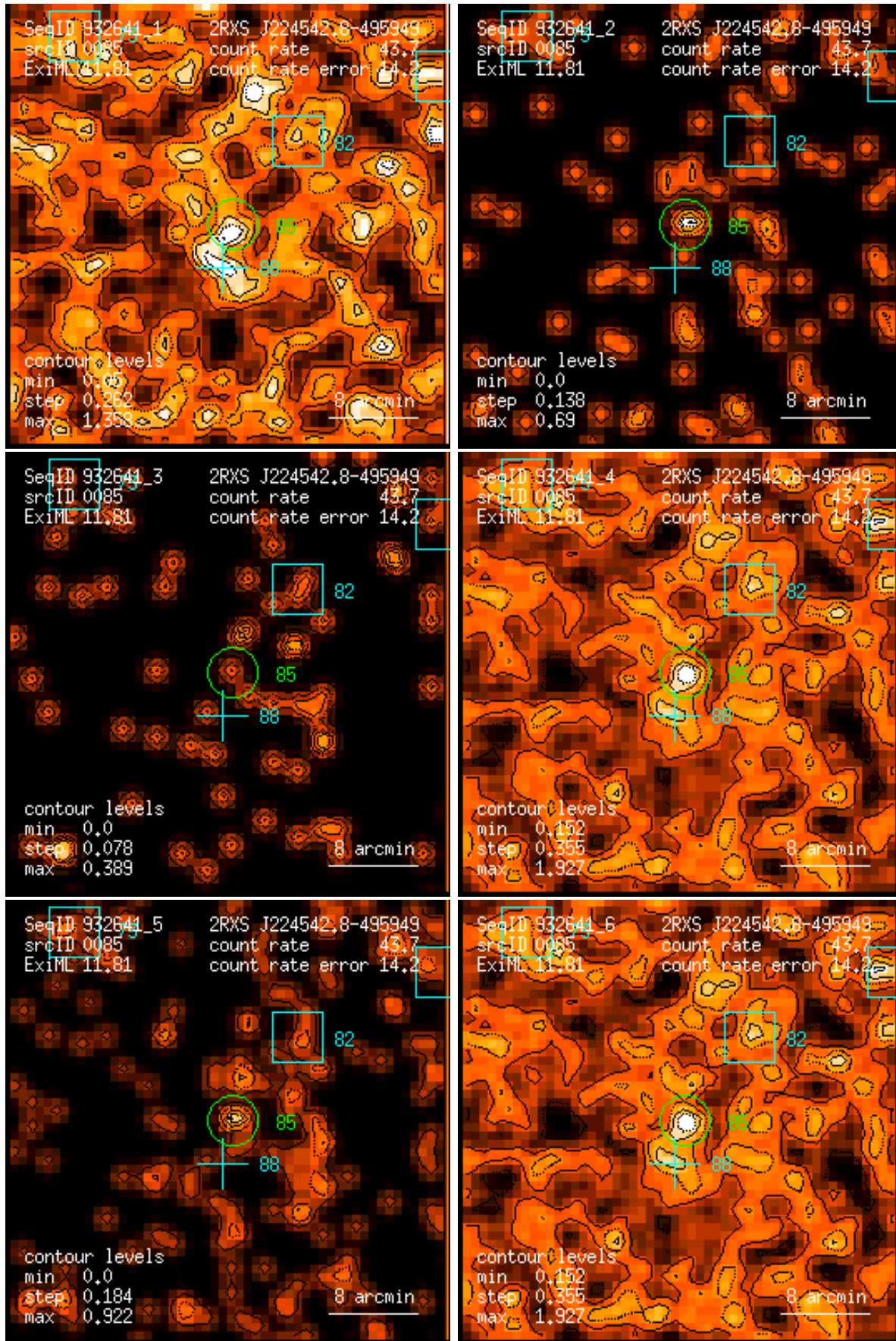
Figure 85: RASS 932641: detection 0085: band rate images, Gaussian filter: (1) PSPC channels 11 – 41, (2) 52 – 90, (3) 91 – 201, (4) 11 – 235, (5) 52 – 201, (6) 11 – 201. Broad band rates in counts/ks. Band rate contour levels in counts/ks/arcmin 2 .
