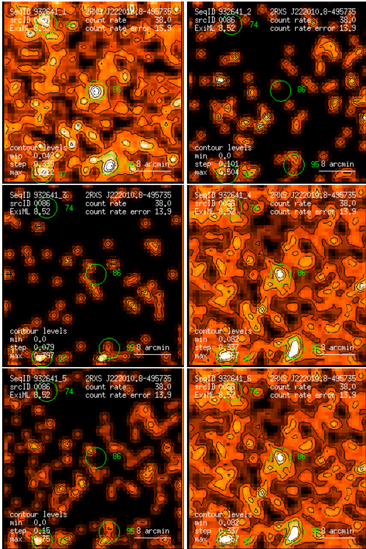
Figure 86: RASS 932641: detection 0086: band rate images, Gaussian filter: (1) PSPC channels 11 – 41, (2) 52 – 90, (3) 91 – 201, (4) 11 – 235, (5) 52 – 201, (6) 11 – 201. Broad band rates in counts/ks. Band rate contour levels in counts/ks/arcmin 2 .
