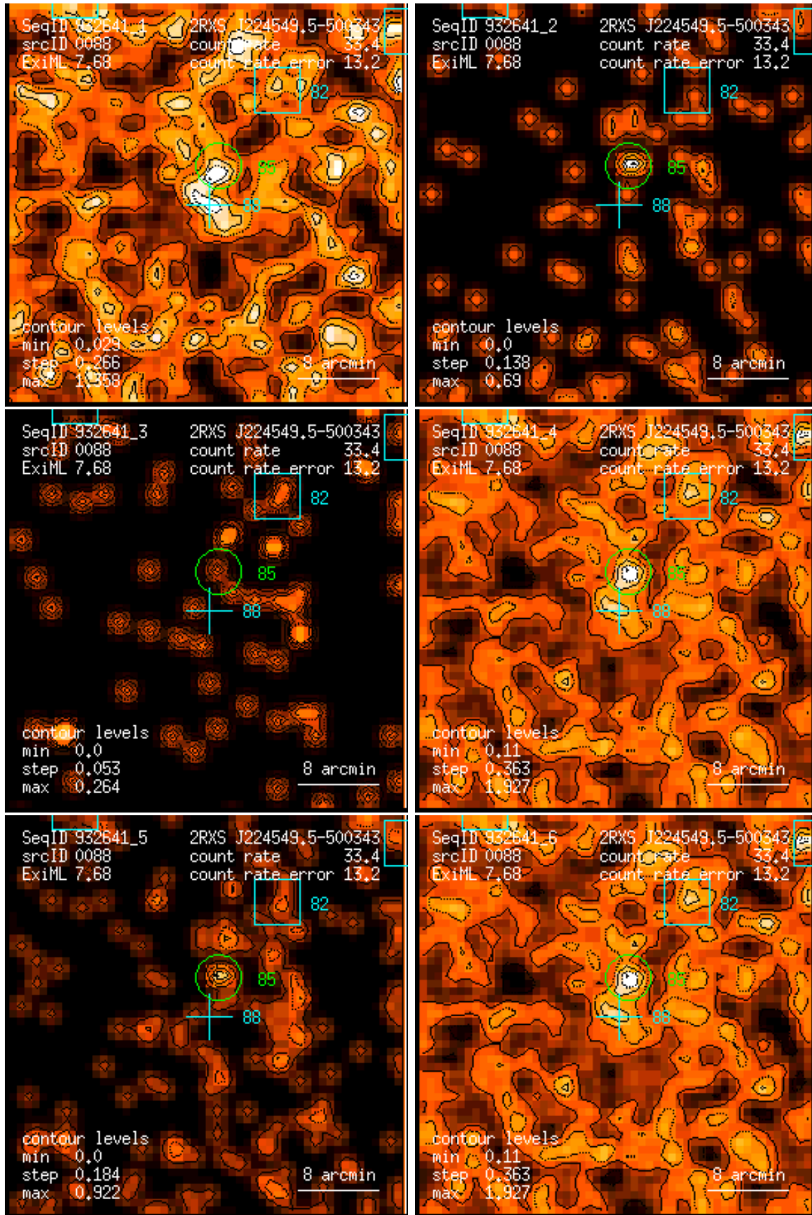
Figure 88: RASS 932641: detection 0088: band rate images, Gaussian filter: (1) PSPC channels 11 – 41, (2) 52 – 90, (3) 91 – 201, (4) 11 – 235, (5) 52 – 201, (6) 11 – 201. Broad band rates in counts/ks. Band rate contour levels in counts/ks/arcmin 2 .
