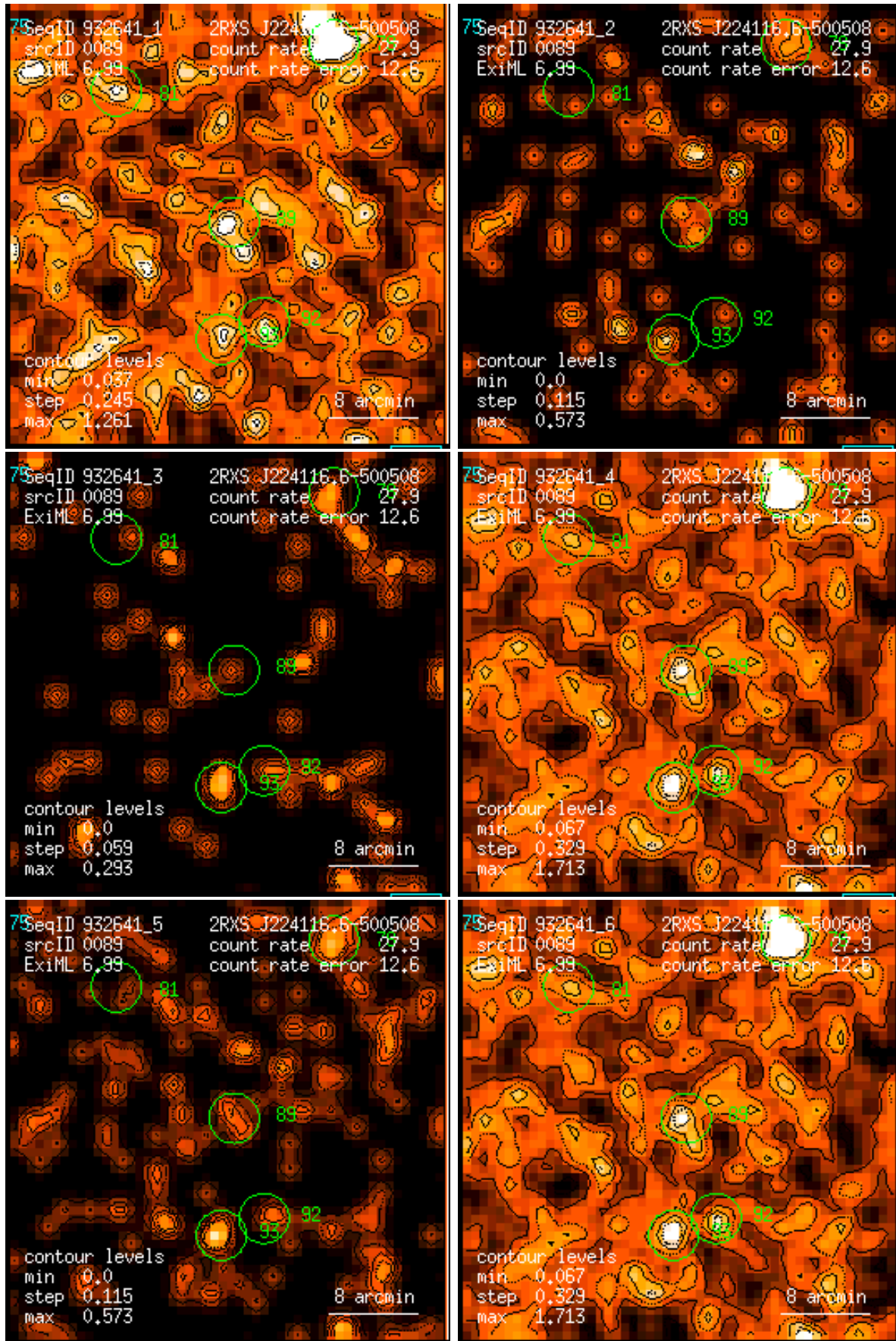
Figure 89: RASS 932641: detection 0089: band rate images, Gaussian filter: (1) PSPC channels 11 – 41, (2) 52 – 90, (3) 91 – 201, (4) 11 – 235, (5) 52 – 201, (6) 11 – 201. Broad band rates in counts/ks. Band rate contour levels in counts/ks/arcmin 2 .
