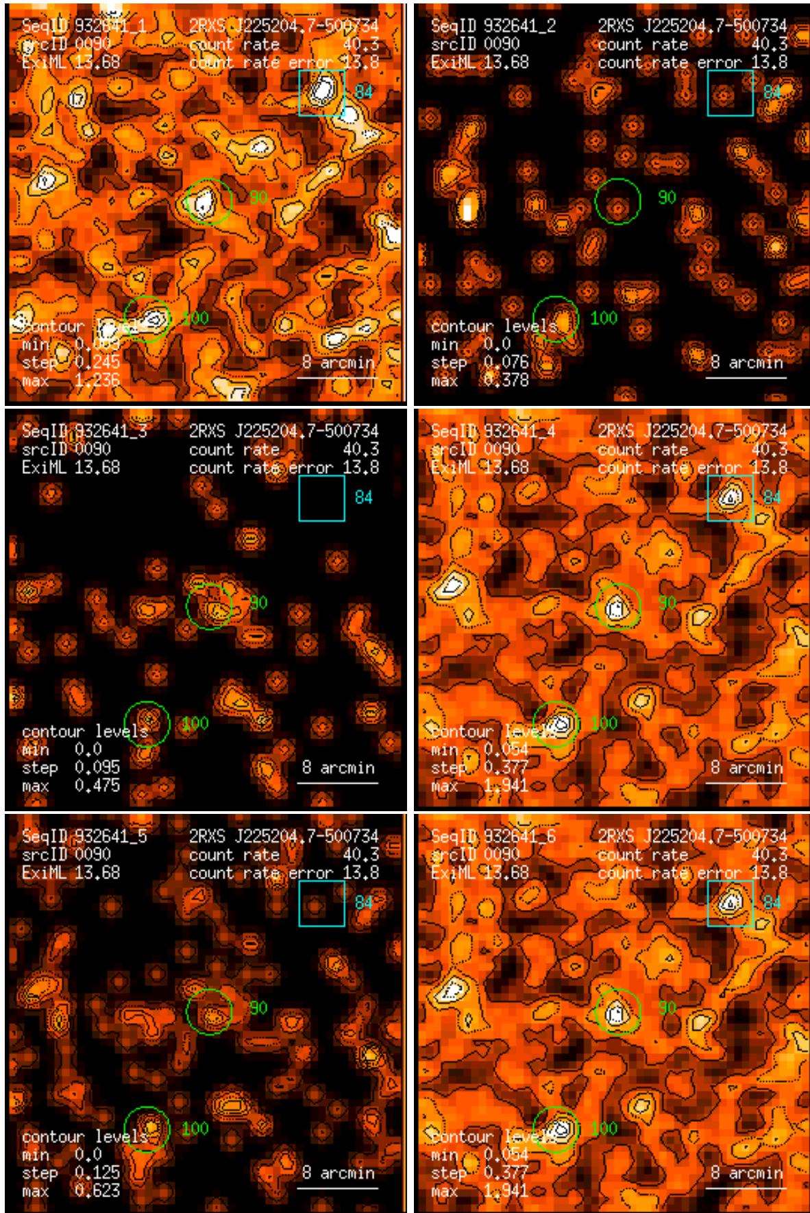
Figure 90: RASS 932641: detection 0090: band rate images, Gaussian filter: (1) PSPC channels 11 – 41, (2) 52 – 90, (3) 91 – 201, (4) 11 – 235, (5) 52 – 201, (6) 11 – 201. Broad band rates in counts/ks. Band rate contour levels in counts/ks/arcmin 2 .
