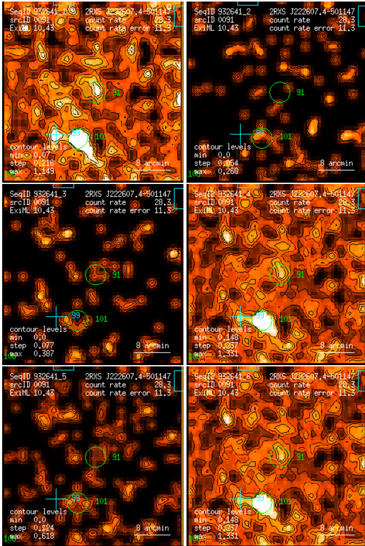
Figure 91: RASS 932641: detection 0091: band rate images, Gaussian filter: (1) PSPC channels 11 – 41, (2) 52 – 90, (3) 91 – 201, (4) 11 – 235, (5) 52 – 201, (6) 11 – 201. Broad band rates in counts/ks. Band rate contour levels in counts/ks/arcmin 2 .
