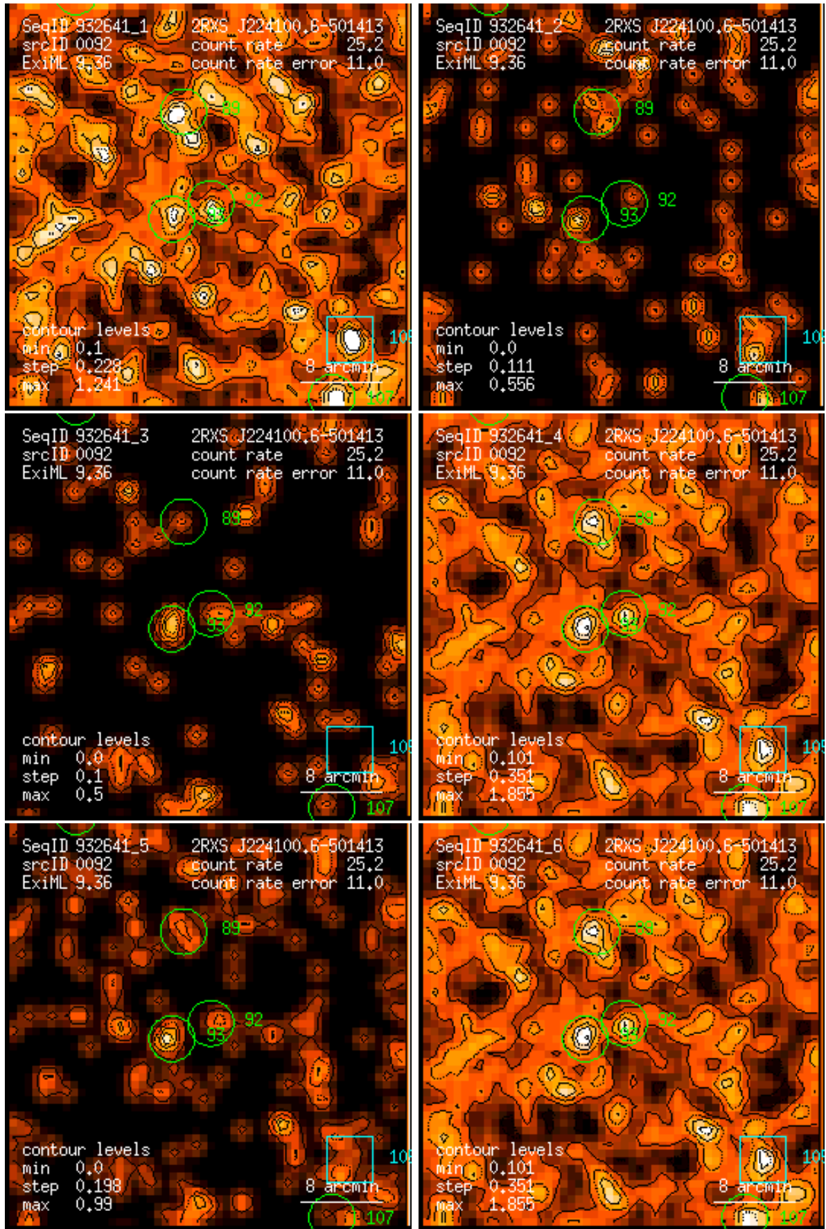
Figure 92: RASS 932641: detection 0092: band rate images, Gaussian filter: (1) PSPC channels 11 – 41, (2) 52 – 90, (3) 91 – 201, (4) 11 – 235, (5) 52 – 201, (6) 11 – 201. Broad band rates in counts/ks. Band rate contour levels in counts/ks/arcmin 2 .
