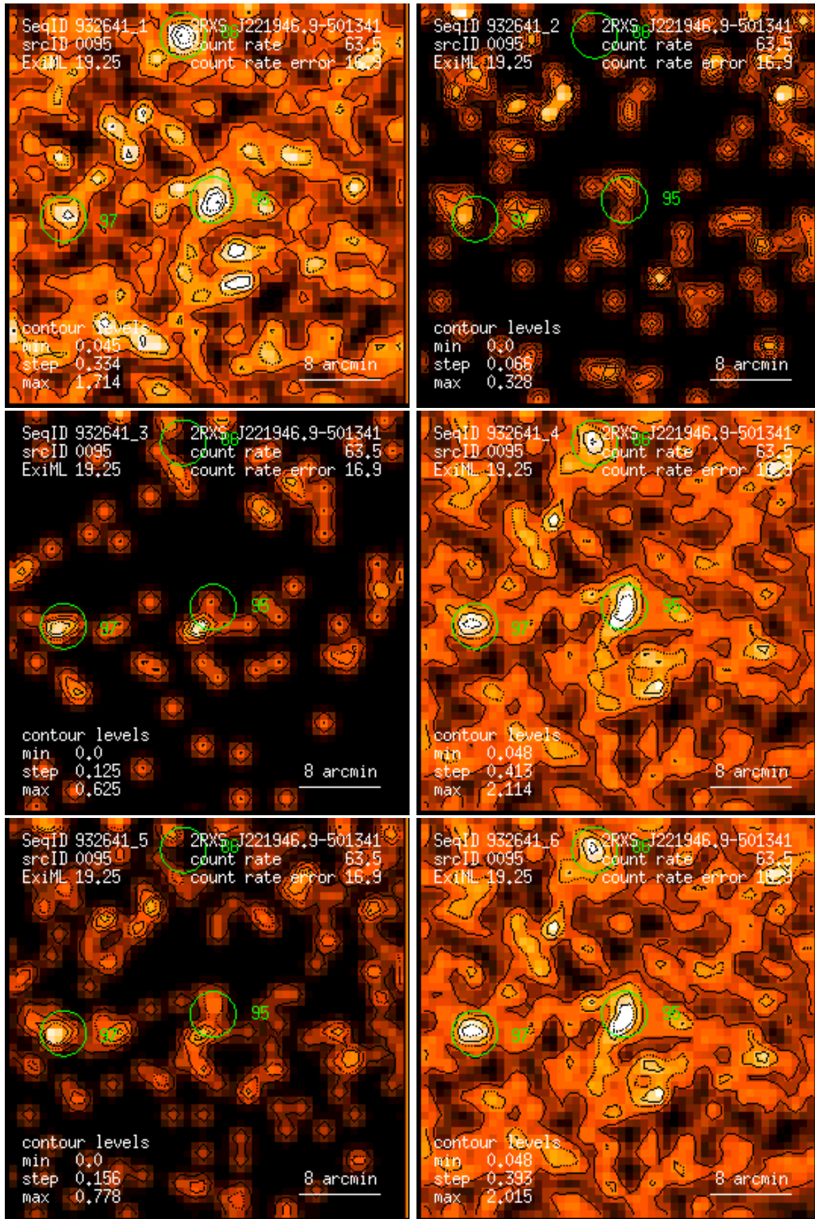
Figure 95: RASS 932641: detection 0095: band rate images, Gaussian filter: (1) PSPC channels 11 – 41, (2) 52 – 90, (3) 91 – 201, (4) 11 – 235, (5) 52 – 201, (6) 11 – 201. Broad band rates in counts/ks. Band rate contour levels in counts/ks/arcmin 2 .
