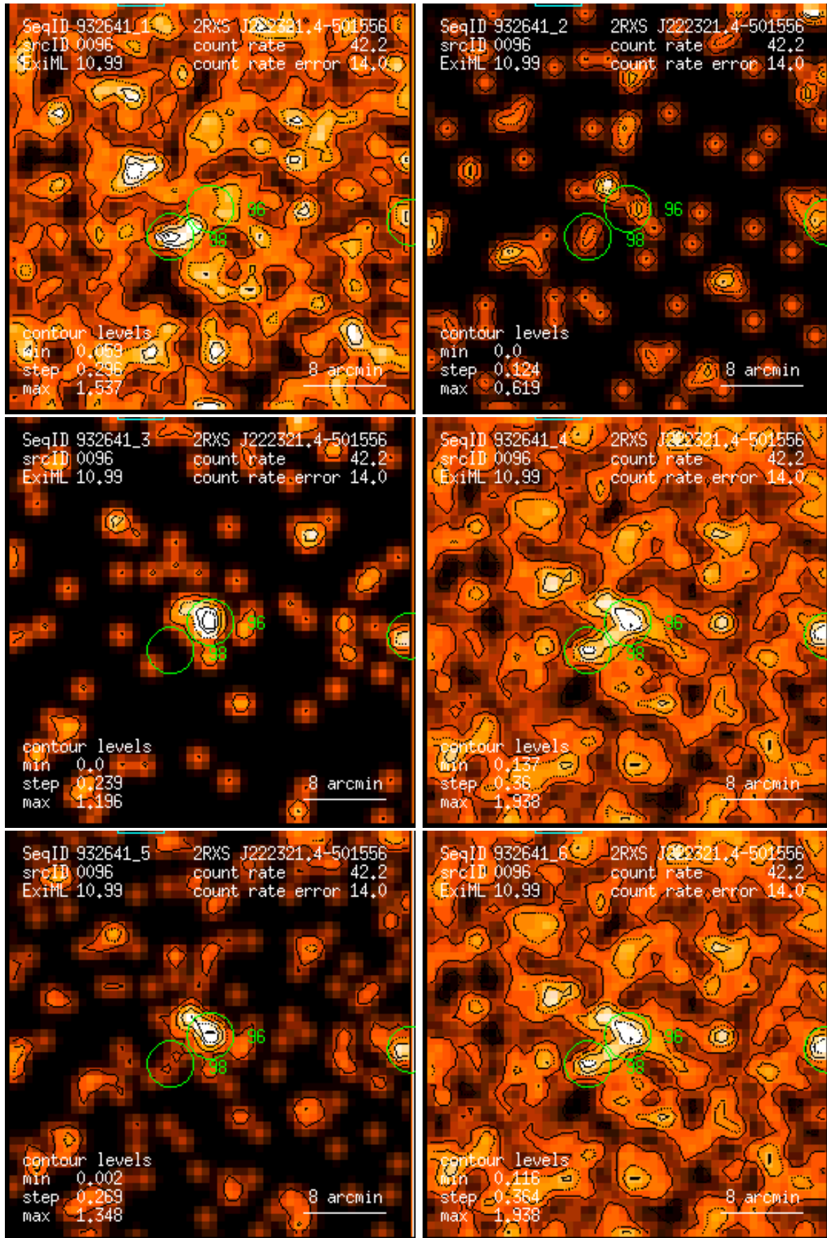
Figure 96: RASS 932641: detection 0096: band rate images, Gaussian filter: (1) PSPC channels 11 – 41, (2) 52 – 90, (3) 91 – 201, (4) 11 – 235, (5) 52 – 201, (6) 11 – 201. Broad band rates in counts/ks. Band rate contour levels in counts/ks/arcmin 2 .
