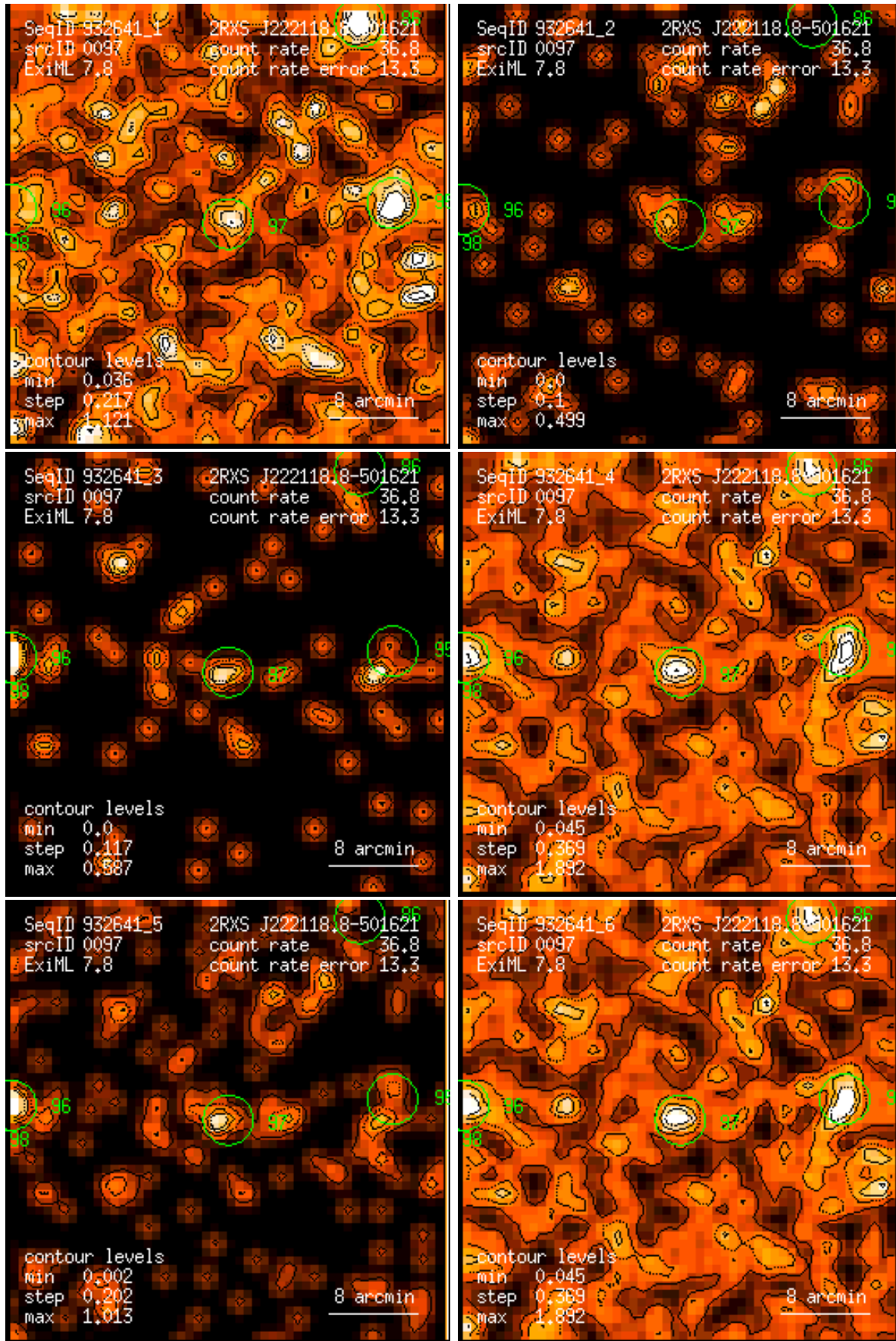
Figure 97: RASS 932641: detection 0097: band rate images, Gaussian filter: (1) PSPC channels 11 – 41, (2) 52 – 90, (3) 91 – 201, (4) 11 – 235, (5) 52 – 201, (6) 11 – 201. Broad band rates in counts/ks. Band rate contour levels in counts/ks/arcmin 2 .
