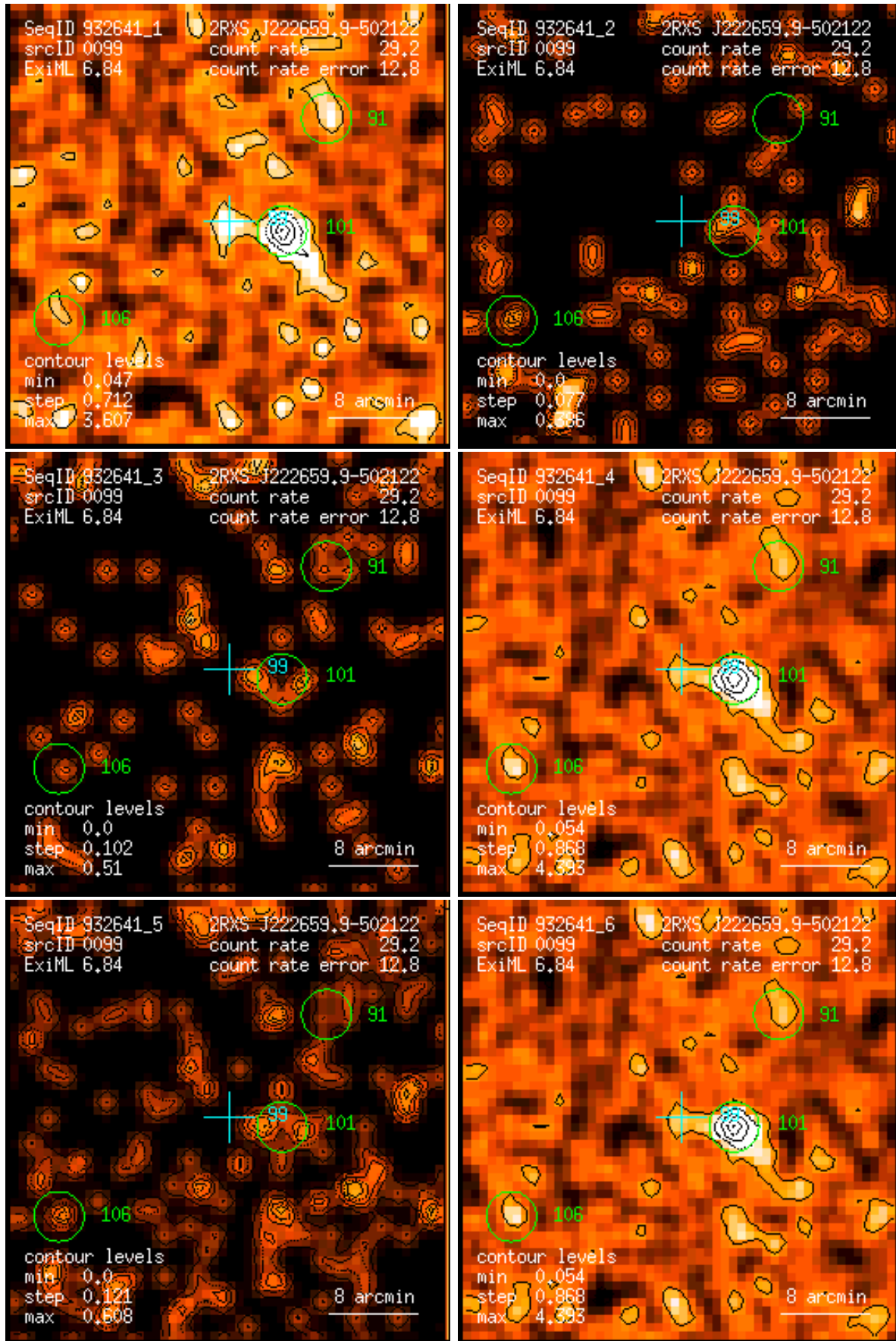
Figure 99: RASS 932641: detection 0099: band rate images, Gaussian filter: (1) PSPC channels 11 – 41, (2) 52 – 90, (3) 91 – 201, (4) 11 – 235, (5) 52 – 201, (6) 11 – 201. Broad band rates in counts/ks. Band rate contour levels in counts/ks/arcmin 2 .
