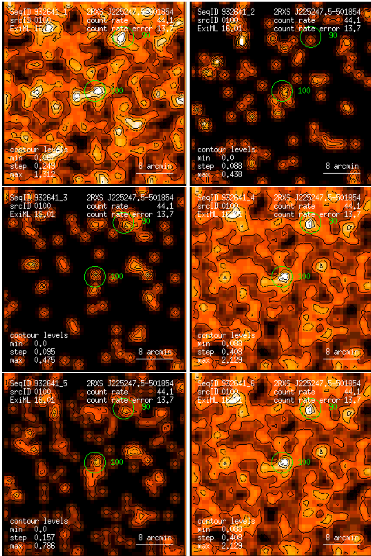
Figure 100: RASS 932641: detection 0100: band rate images, Gaussian filter: (1) PSPC channels 11 – 41, (2) 52 – 90, (3) 91 – 201, (4) 11 – 235, (5) 52 – 201, (6) 11 – 201. Broad band rates in counts/ks. Band rate contour levels in counts/ks/arcmin 2 .
