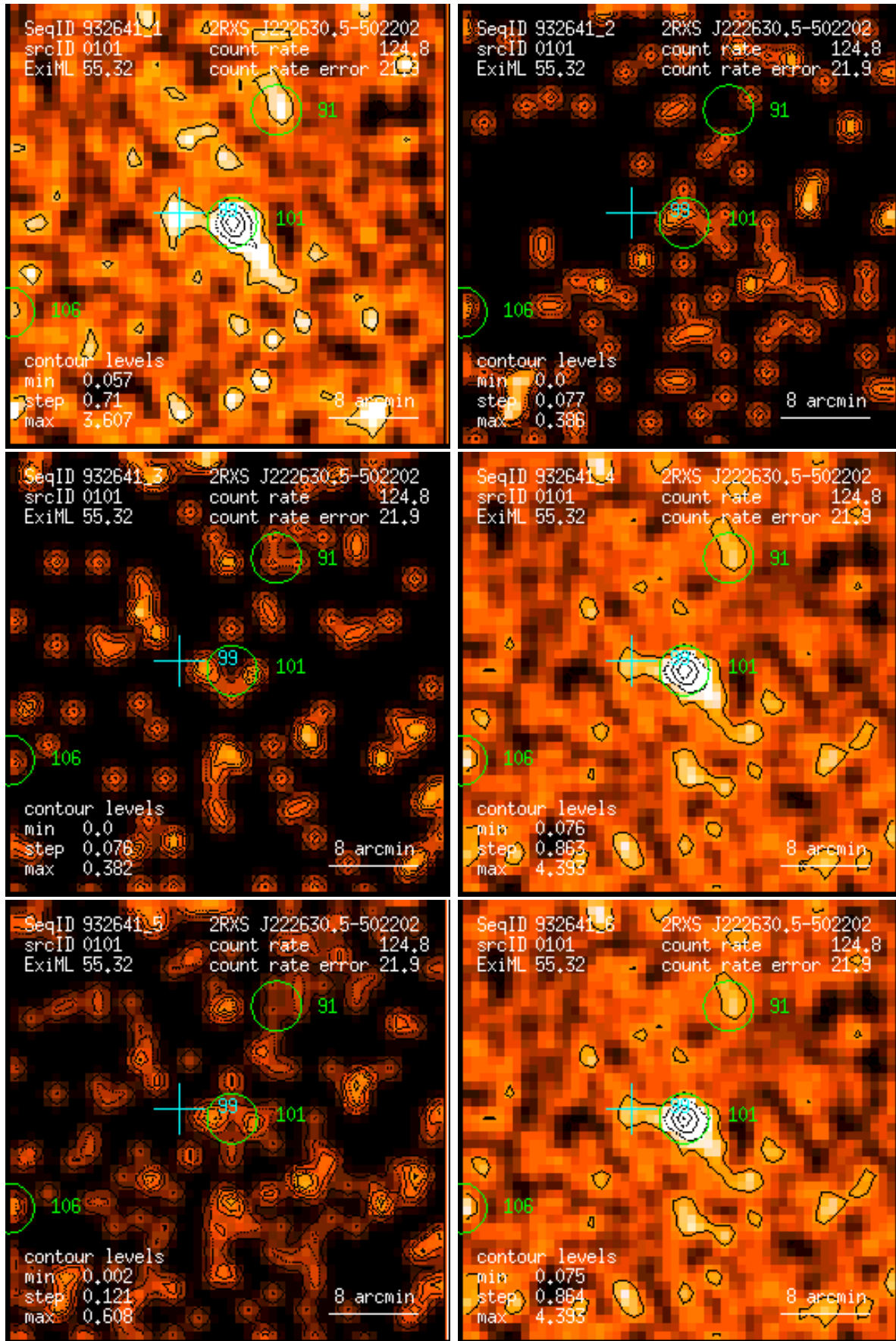
Figure 101: RASS 932641: detection 0101: band rate images, Gaussian filter: (1) PSPC channels 11 – 41, (2) 52 – 90, (3) 91 – 201, (4) 11 – 235, (5) 52 – 201, (6) 11 – 201. Broad band rates in counts/ks. Band rate contour levels in counts/ks/arcmin 2 .
