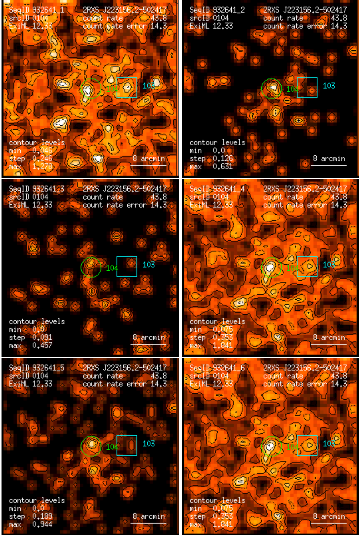
Figure 104: RASS 932641: detection 0104: band rate images, Gaussian filter: (1) PSPC channels 11 – 41, (2) 52 – 90, (3) 91 – 201, (4) 11 – 235, (5) 52 – 201, (6) 11 – 201. Broad band rates in counts/ks. Band rate contour levels in counts/ks/arcmin 2 .
