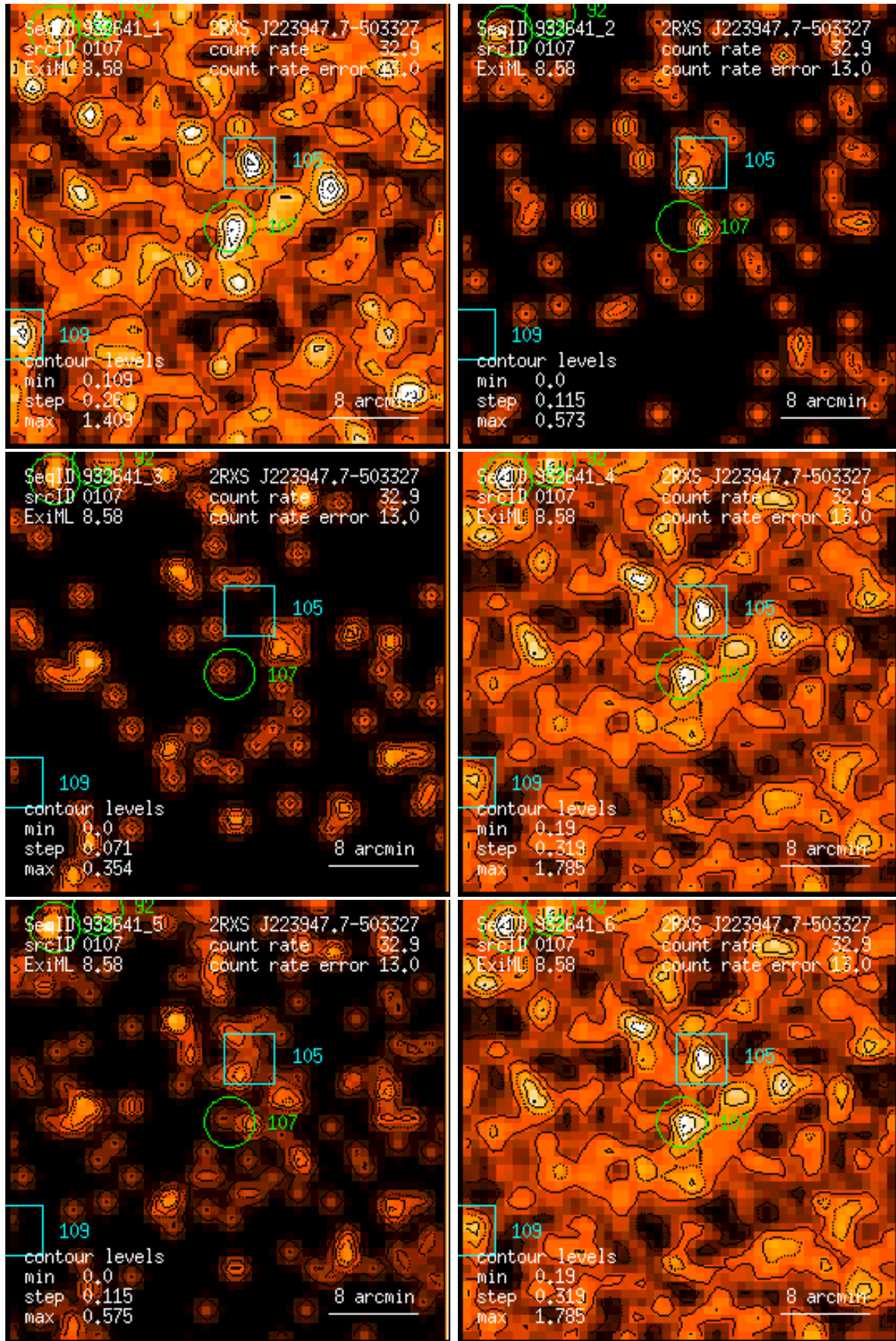
Figure 107: RASS 932641: detection 0107: band rate images, Gaussian filter: (1) PSPC channels 11 – 41, (2) 52 – 90, (3) 91 – 201, (4) 11 – 235, (5) 52 – 201, (6) 11 – 201. Broad band rates in counts/ks. Band rate contour levels in counts/ks/arcmin 2 .
