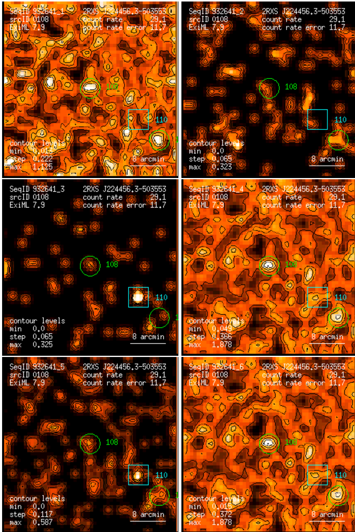
Figure 108: RASS 932641: detection 0108: band rate images, Gaussian filter: (1) PSPC channels 11 – 41, (2) 52 – 90, (3) 91 – 201, (4) 11 – 235, (5) 52 – 201, (6) 11 – 201. Broad band rates in counts/ks. Band rate contour levels in counts/ks/arcmin 2 .
