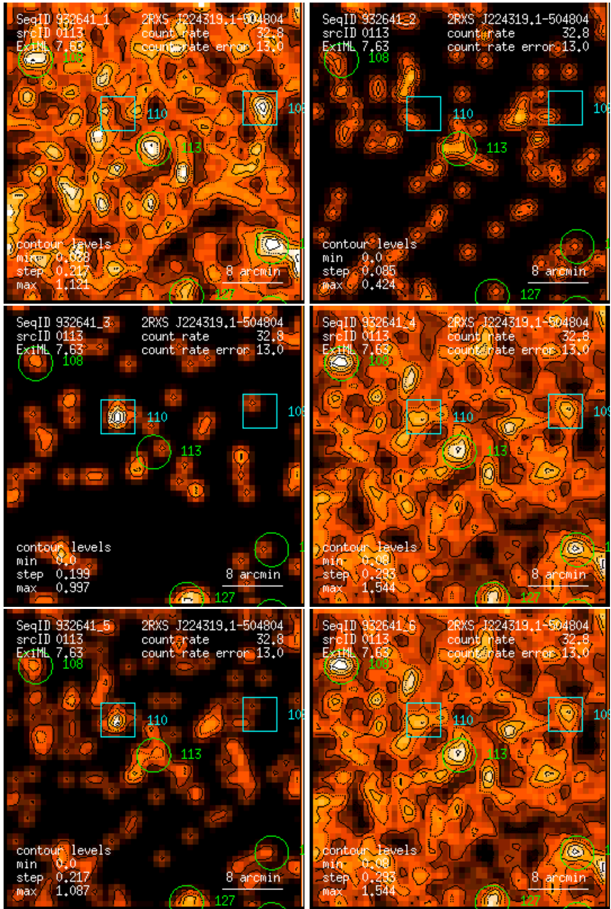
Figure 113: RASS 932641: detection 0113: band rate images, Gaussian filter: (1) PSPC channels 11 – 41, (2) 52 – 90, (3) 91 – 201, (4) 11 – 235, (5) 52 – 201, (6) 11 – 201. Broad band rates in counts/ks. Band rate contour levels in counts/ks/arcmin 2 .
