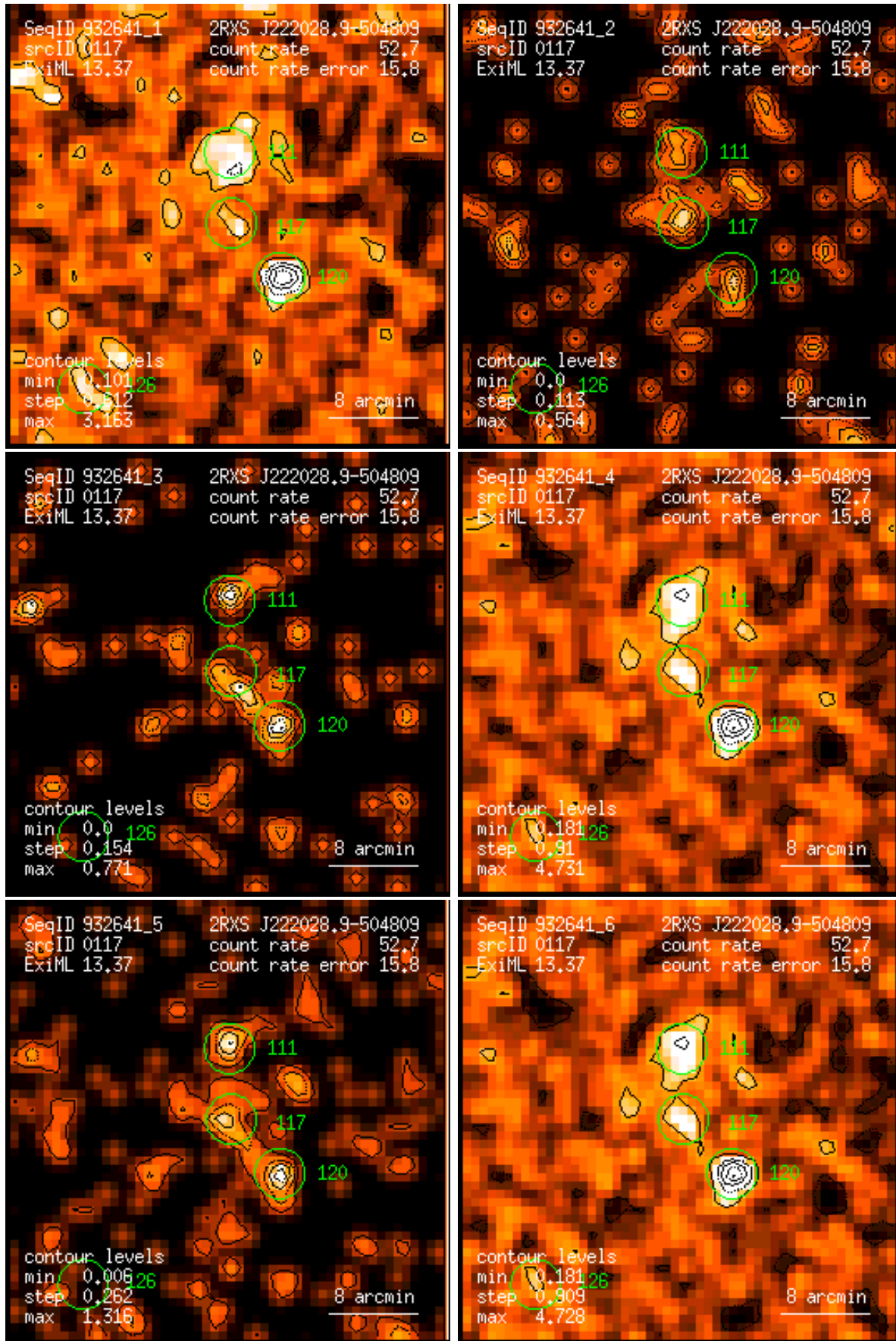
Figure 117: RASS 932641: detection 0117: band rate images, Gaussian filter: (1) PSPC channels 11 – 41, (2) 52 – 90, (3) 91 – 201, (4) 11 – 235, (5) 52 – 201, (6) 11 – 201. Broad band rates in counts/ks. Band rate contour levels in counts/ks/arcmin 2 .
