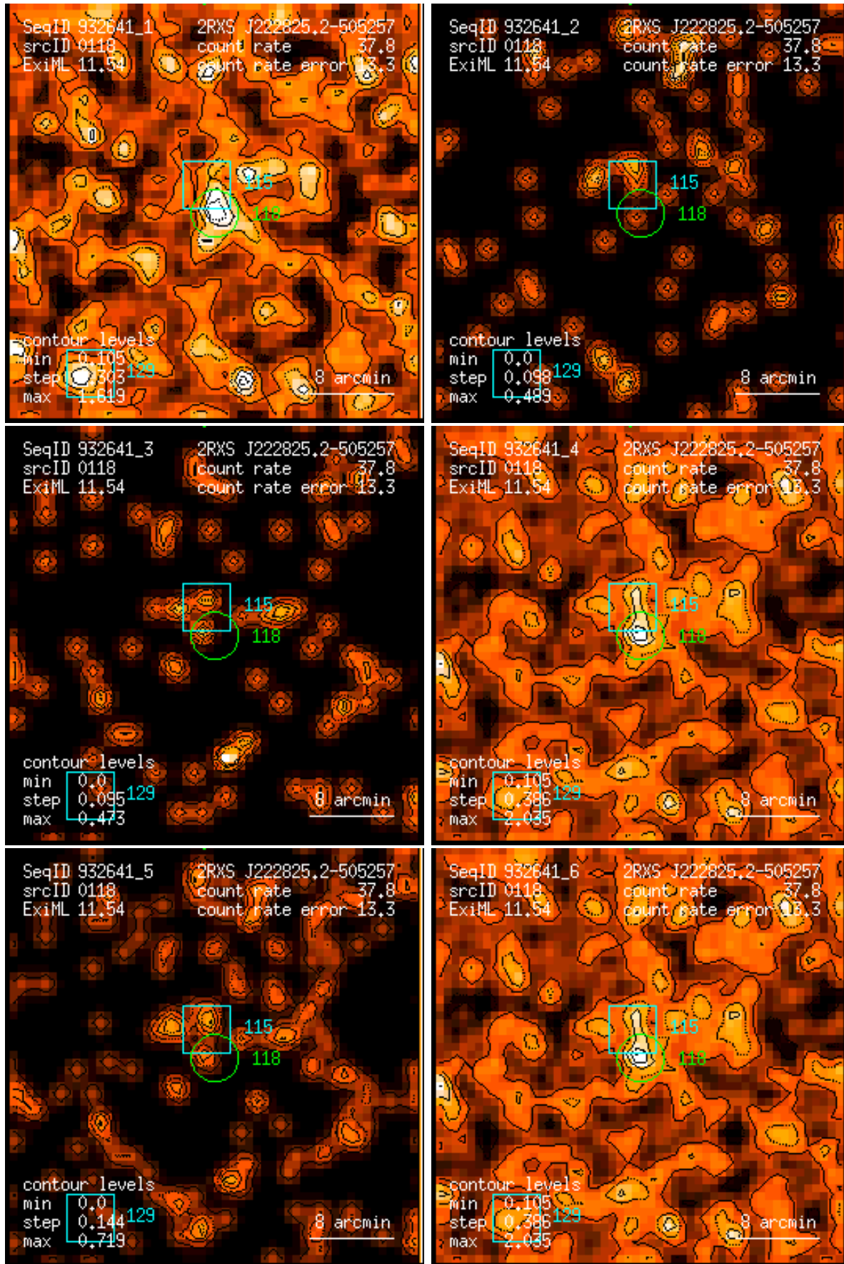
Figure 118: RASS 932641: detection 0118: band rate images, Gaussian filter: (1) PSPC channels 11 – 41, (2) 52 – 90, (3) 91 – 201, (4) 11 – 235, (5) 52 – 201, (6) 11 – 201. Broad band rates in counts/ks. Band rate contour levels in counts/ks/arcmin 2 .
