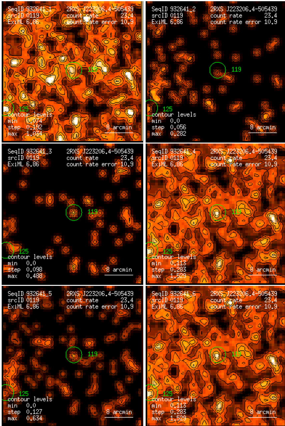
Figure 119: RASS 932641: detection 0119: band rate images, Gaussian filter: (1) PSPC channels 11 – 41, (2) 52 – 90, (3) 91 – 201, (4) 11 – 235, (5) 52 – 201, (6) 11 – 201. Broad band rates in counts/ks. Band rate contour levels in counts/ks/arcmin 2 .
