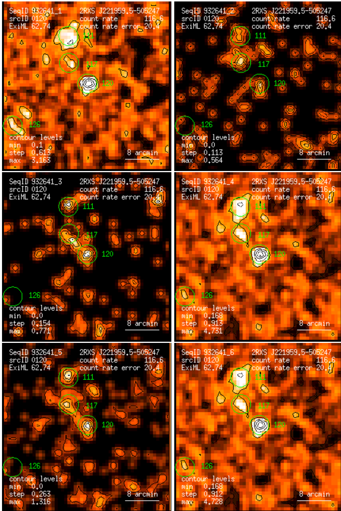
Figure 120: RASS 932641: detection 0120: band rate images, Gaussian filter: (1) PSPC channels 11 – 41, (2) 52 – 90, (3) 91 – 201, (4) 11 – 235, (5) 52 – 201, (6) 11 – 201. Broad band rates in counts/ks. Band rate contour levels in counts/ks/arcmin 2 .
