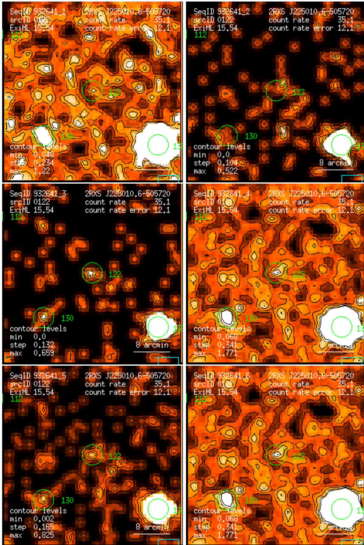
Figure 122: RASS 932641: detection 0122: band rate images, Gaussian filter: (1) PSPC channels 11 – 41, (2) 52 – 90, (3) 91 – 201, (4) 11 – 235, (5) 52 – 201, (6) 11 – 201. Broad band rates in counts/ks. Band rate contour levels in counts/ks/arcmin 2 .
