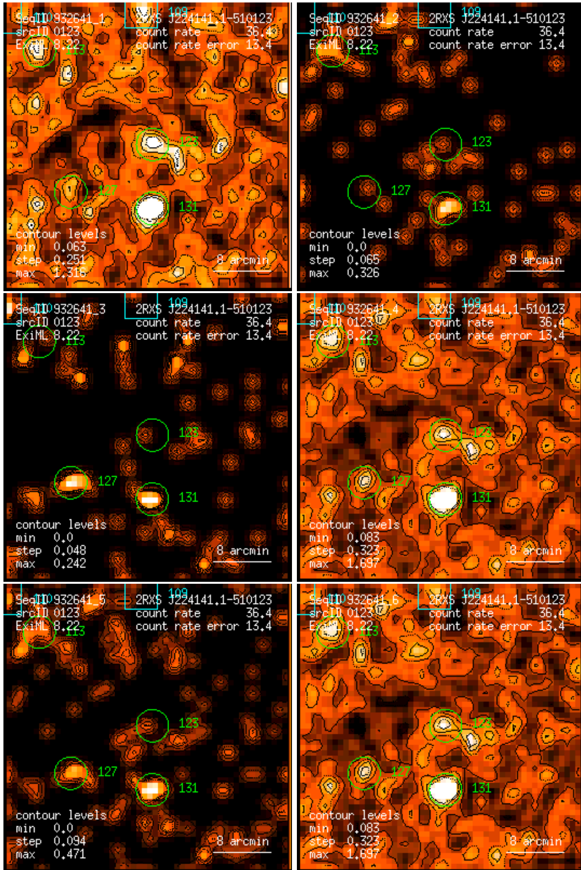
Figure 123: RASS 932641: detection 0123: band rate images, Gaussian filter: (1) PSPC channels 11 – 41, (2) 52 – 90, (3) 91 – 201, (4) 11 – 235, (5) 52 – 201, (6) 11 – 201. Broad band rates in counts/ks. Band rate contour levels in counts/ks/arcmin 2 .
