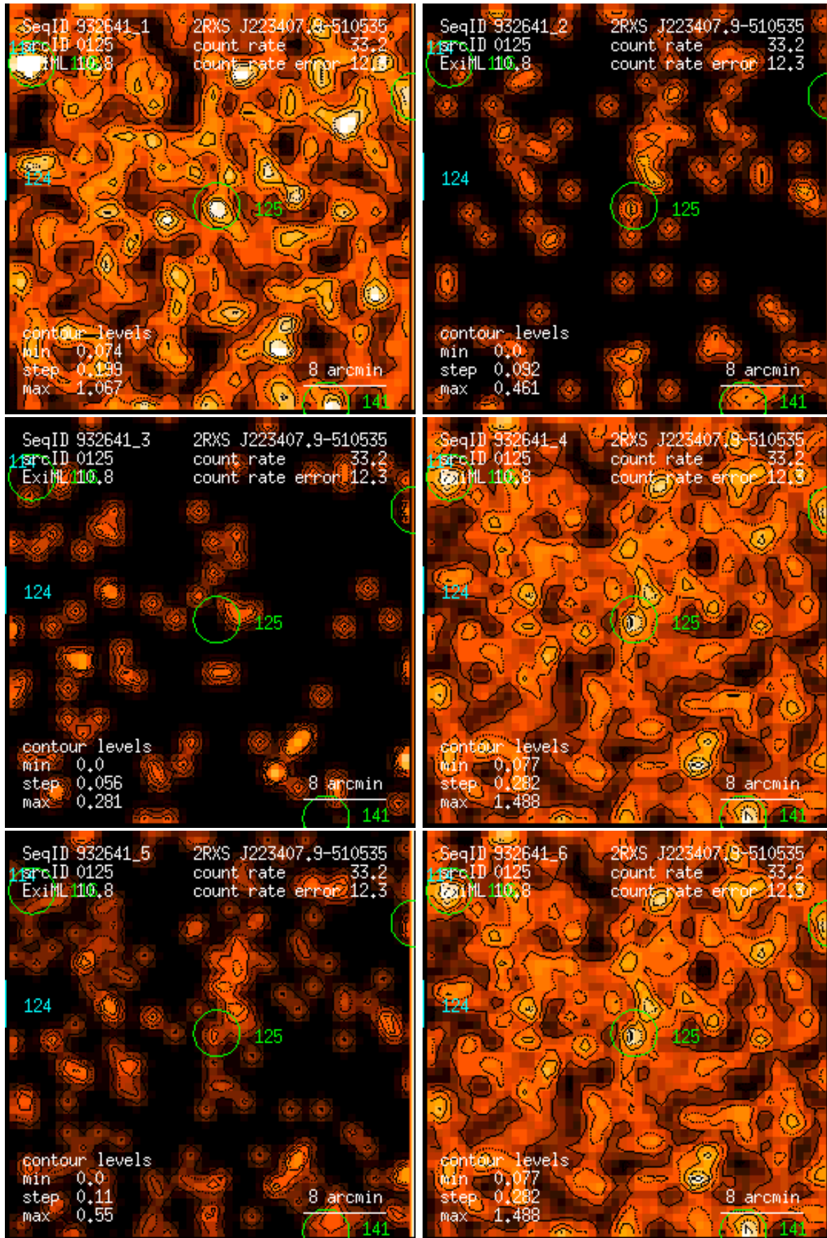
Figure 125: RASS 932641: detection 0125: band rate images, Gaussian filter: (1) PSPC channels 11 – 41, (2) 52 – 90, (3) 91 – 201, (4) 11 – 235, (5) 52 – 201, (6) 11 – 201. Broad band rates in counts/ks. Band rate contour levels in counts/ks/arcmin 2 .
