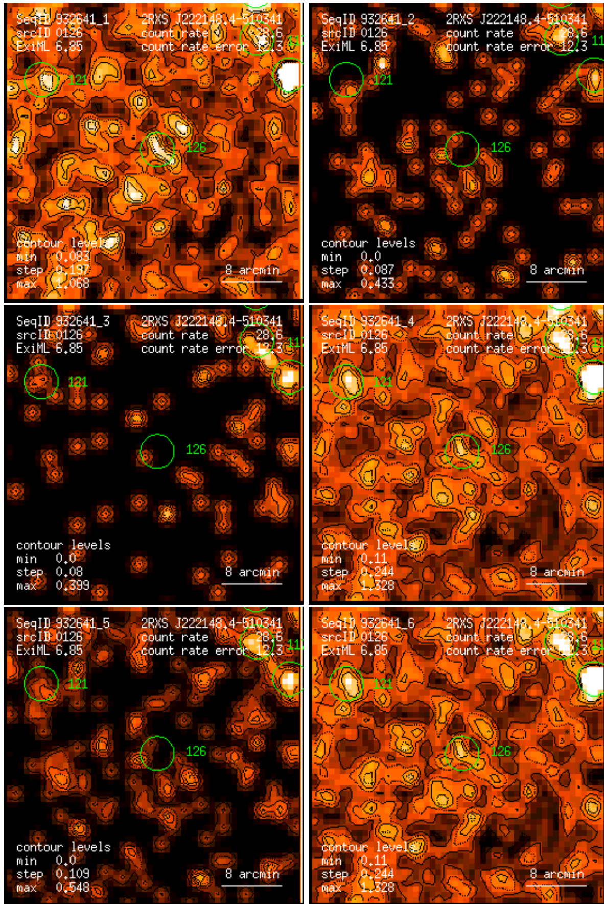
Figure 126: RASS 932641: detection 0126: band rate images, Gaussian filter: (1) PSPC channels 11 – 41, (2) 52 – 90, (3) 91 – 201, (4) 11 – 235, (5) 52 – 201, (6) 11 – 201. Broad band rates in counts/ks. Band rate contour levels in counts/ks/arcmin 2 .
