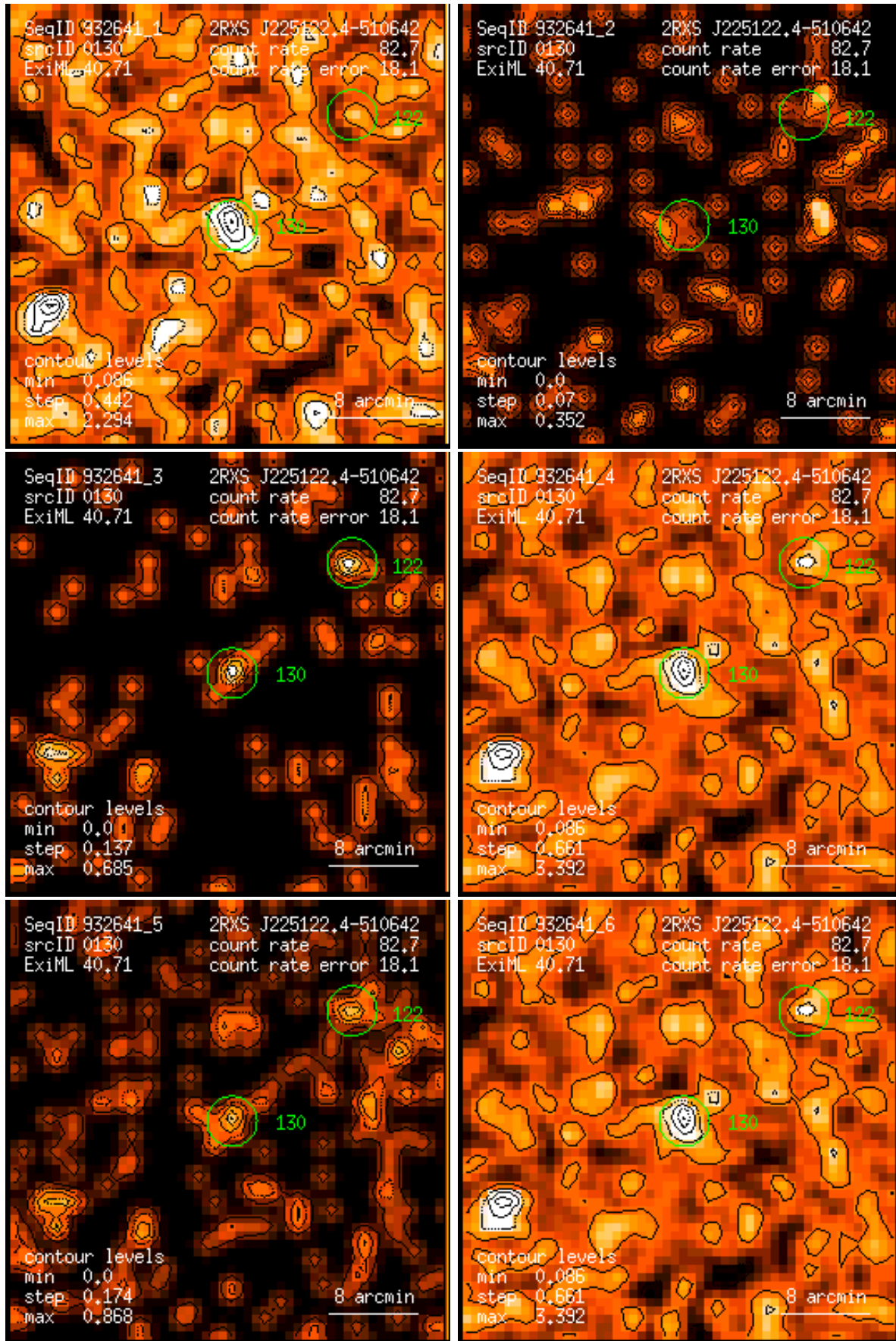
Figure 130: RASS 932641: detection 0130: band rate images, Gaussian filter: (1) PSPC channels 11 – 41, (2) 52 – 90, (3) 91 – 201, (4) 11 – 235, (5) 52 – 201, (6) 11 – 201. Broad band rates in counts/ks. Band rate contour levels in counts/ks/arcmin 2 .
