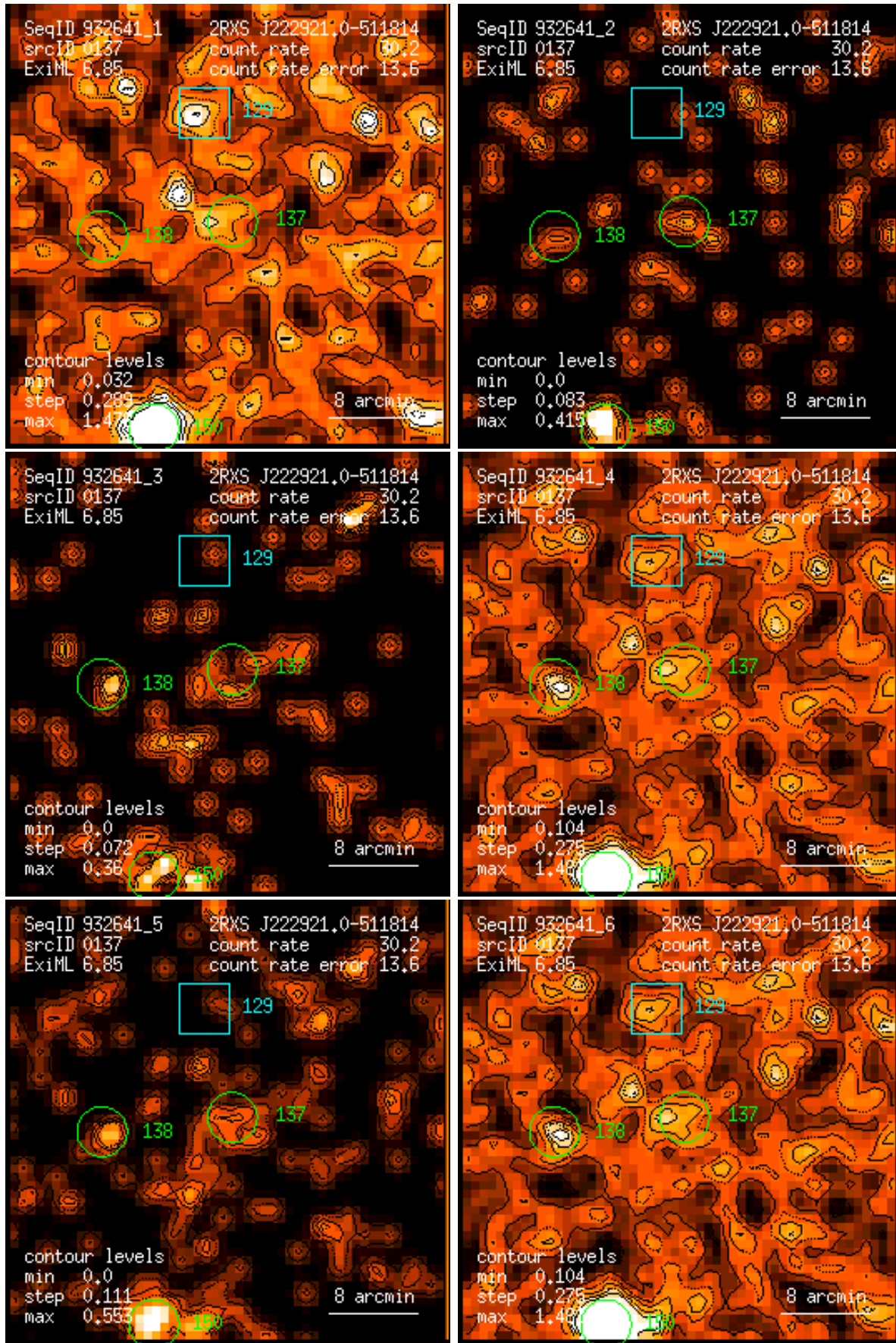
Figure 137: RASS 932641: detection 0137: band rate images, Gaussian filter: (1) PSPC channels 11 – 41, (2) 52 – 90, (3) 91 – 201, (4) 11 – 235, (5) 52 – 201, (6) 11 – 201. Broad band rates in counts/ks. Band rate contour levels in counts/ks/arcmin 2 .
