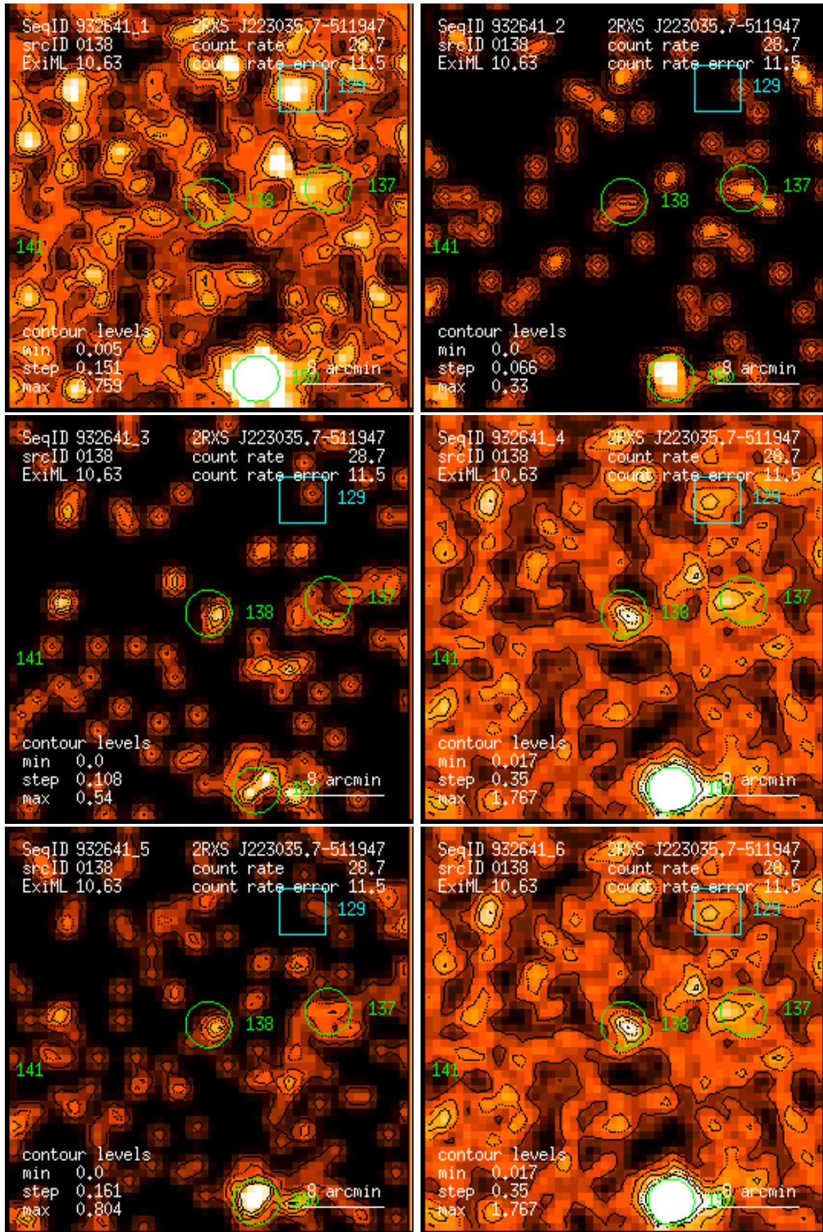
Figure 138: RASS 932641: detection 0138: band rate images, Gaussian filter: (1) PSPC channels 11 – 41, (2) 52 – 90, (3) 91 – 201, (4) 11 – 235, (5) 52 – 201, (6) 11 – 201. Broad band rates in counts/ks. Band rate contour levels in counts/ks/arcmin 2 .
