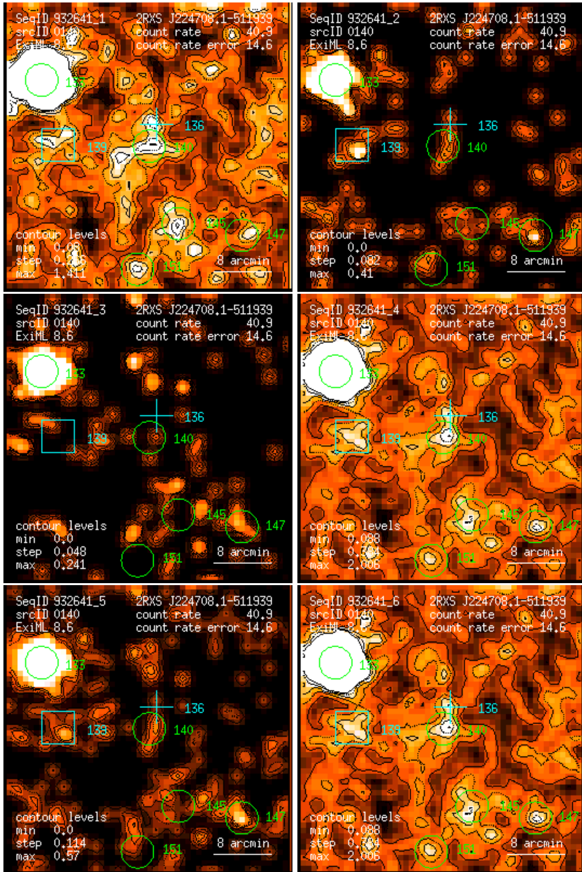
Figure 140: RASS 932641: detection 0140: band rate images, Gaussian filter: (1) PSPC channels 11 – 41, (2) 52 – 90, (3) 91 – 201, (4) 11 – 235, (5) 52 – 201, (6) 11 – 201. Broad band rates in counts/ks. Band rate contour levels in counts/ks/arcmin 2 .
