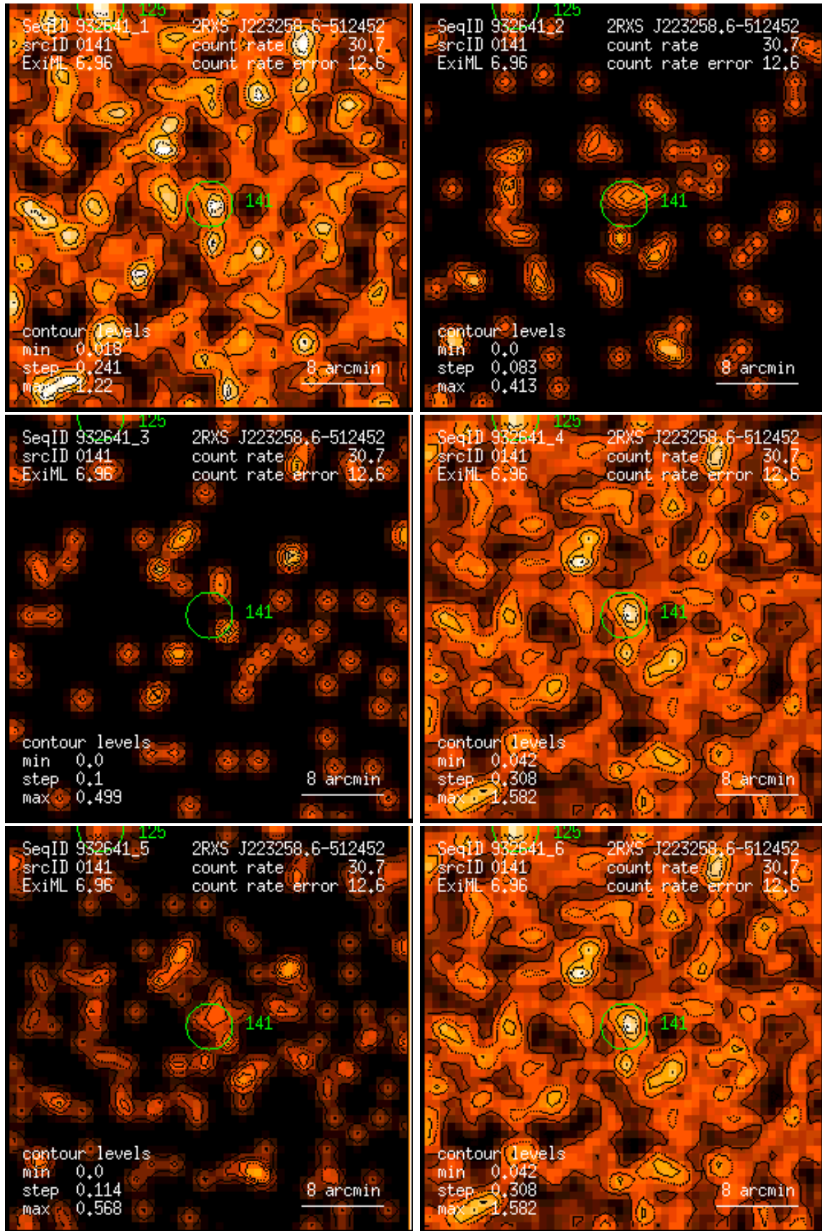
Figure 141: RASS 932641: detection 0141: band rate images, Gaussian filter: (1) PSPC channels 11 – 41, (2) 52 – 90, (3) 91 – 201, (4) 11 – 235, (5) 52 – 201, (6) 11 – 201. Broad band rates in counts/ks. Band rate contour levels in counts/ks/arcmin 2 .
