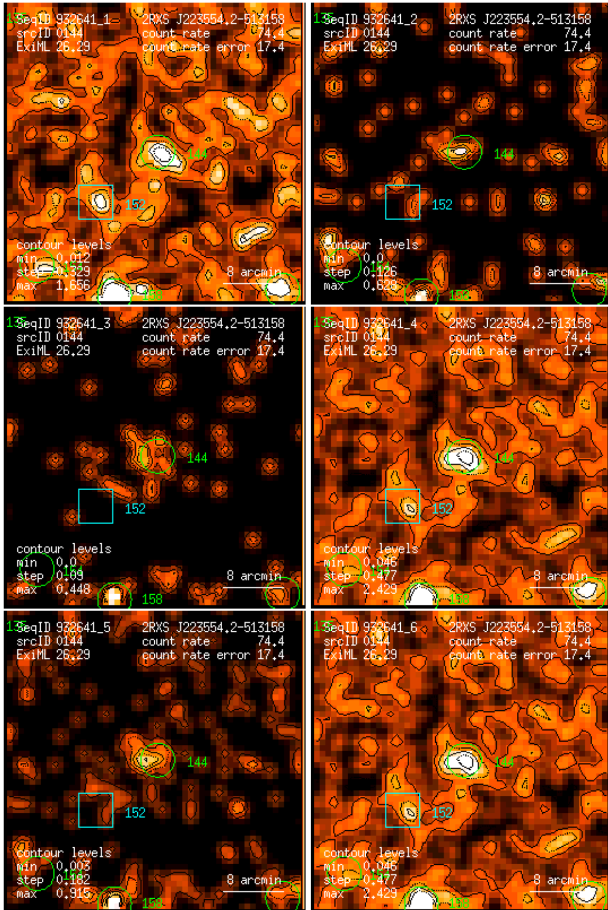
Figure 144: RASS 932641: detection 0144: band rate images, Gaussian filter: (1) PSPC channels 11 – 41, (2) 52 – 90, (3) 91 – 201, (4) 11 – 235, (5) 52 – 201, (6) 11 – 201. Broad band rates in counts/ks. Band rate contour levels in counts/ks/arcmin 2 .
