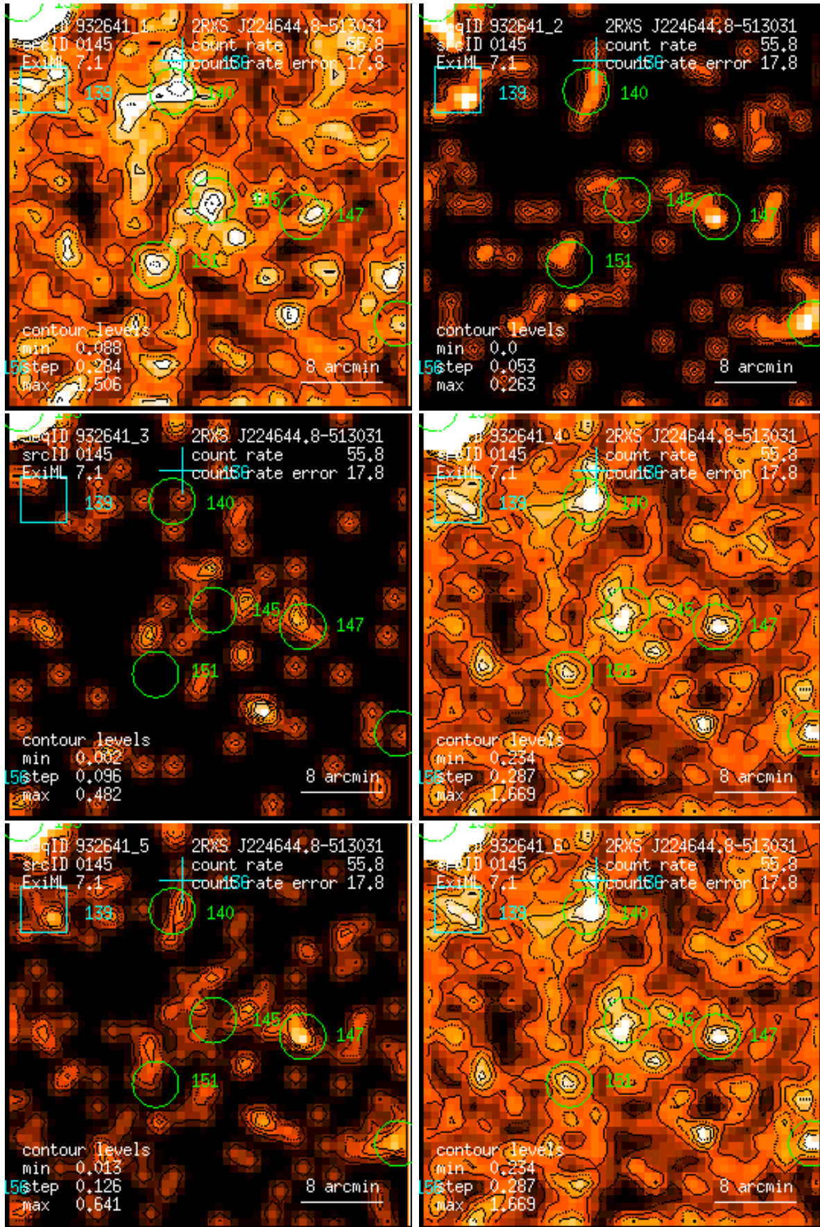
Figure 145: RASS 932641: detection 0145: band rate images, Gaussian filter: (1) PSPC channels 11 – 41, (2) 52 – 90, (3) 91 – 201, (4) 11 – 235, (5) 52 – 201, (6) 11 – 201. Broad band rates in counts/ks. Band rate contour levels in counts/ks/arcmin 2 .
