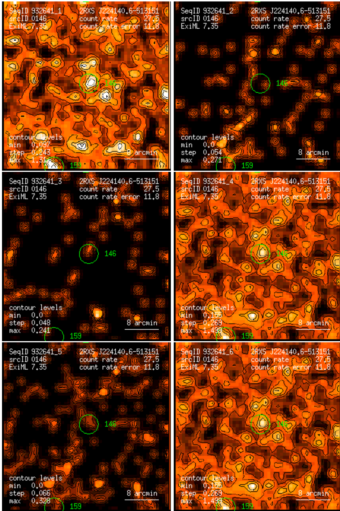
Figure 146: RASS 932641: detection 0146: band rate images, Gaussian filter: (1) PSPC channels 11 – 41, (2) 52 – 90, (3) 91 – 201, (4) 11 – 235, (5) 52 – 201, (6) 11 – 201. Broad band rates in counts/ks. Band rate contour levels in counts/ks/arcmin 2 .
