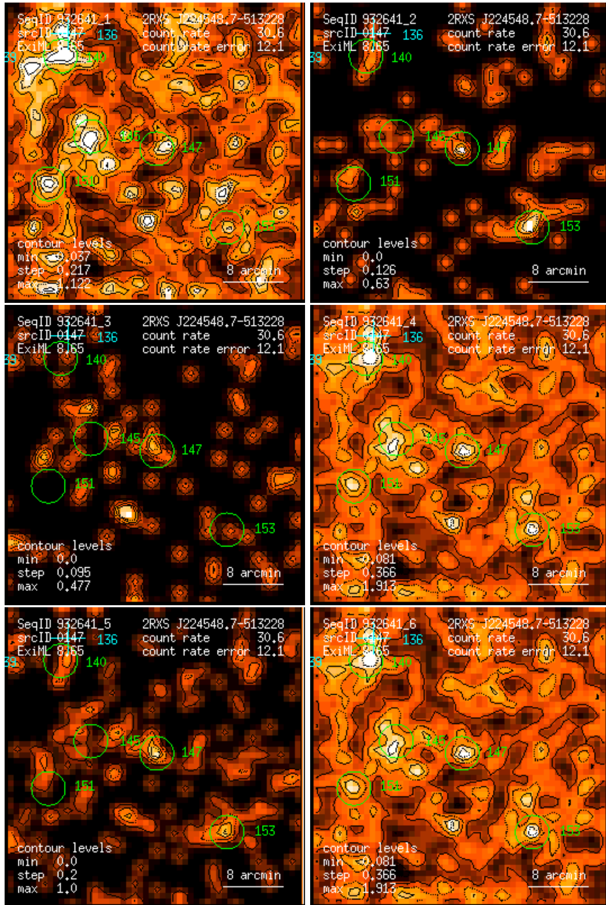
Figure 147: RASS 932641: detection 0147: band rate images, Gaussian filter: (1) PSPC channels 11 – 41, (2) 52 – 90, (3) 91 – 201, (4) 11 – 235, (5) 52 – 201, (6) 11 – 201. Broad band rates in counts/ks. Band rate contour levels in counts/ks/arcmin 2 .
