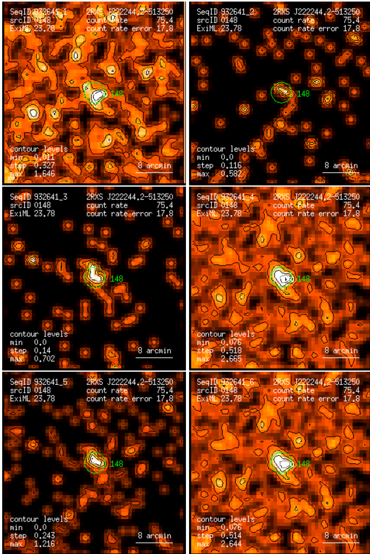
Figure 148: RASS 932641: detection 0148: band rate images, Gaussian filter: (1) PSPC channels 11 – 41, (2) 52 – 90, (3) 91 – 201, (4) 11 – 235, (5) 52 – 201, (6) 11 – 201. Broad band rates in counts/ks. Band rate contour levels in counts/ks/arcmin 2 .
