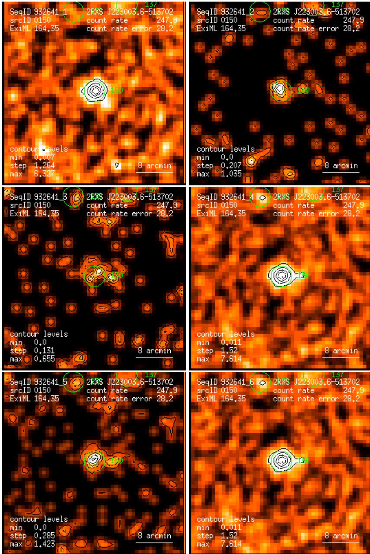
Figure 150: RASS 932641: detection 0150: band rate images, Gaussian filter: (1) PSPC channels 11 – 41, (2) 52 – 90, (3) 91 – 201, (4) 11 – 235, (5) 52 – 201, (6) 11 – 201. Broad band rates in counts/ks. Band rate contour levels in counts/ks/arcmin 2 .
