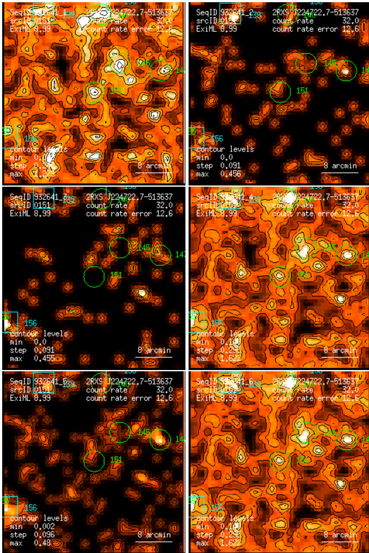
Figure 151: RASS 932641: detection 0151: band rate images, Gaussian filter: (1) PSPC channels 11 – 41, (2) 52 – 90, (3) 91 – 201, (4) 11 – 235, (5) 52 – 201, (6) 11 – 201. Broad band rates in counts/ks. Band rate contour levels in counts/ks/arcmin 2 .
